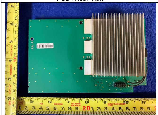
PCB5 Rear View
