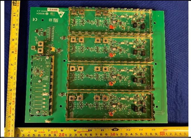
PCB4 Front View
