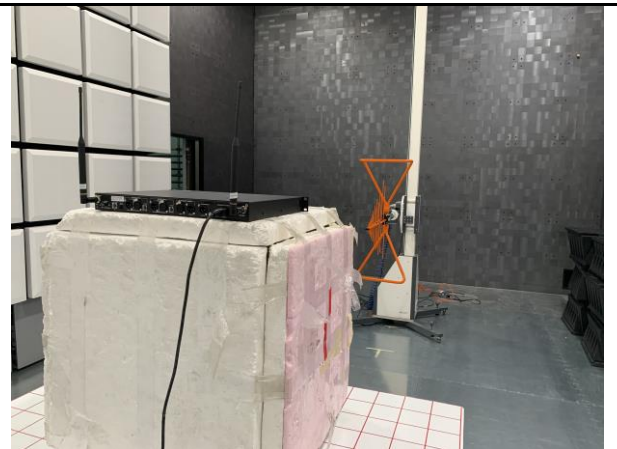
Radiated Emission Test below 30MHz Rear View
