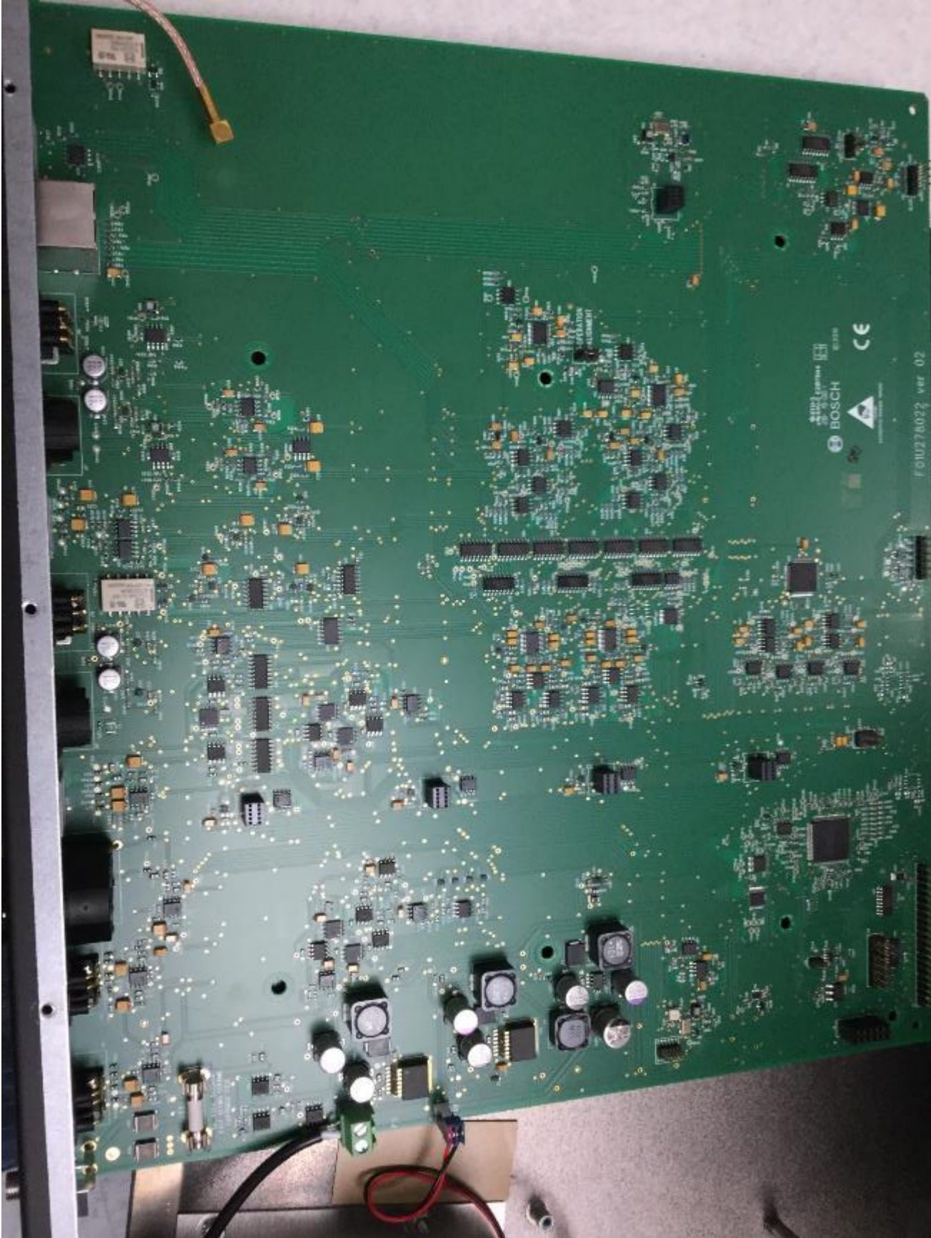
BTR-30N – Internal Photos
