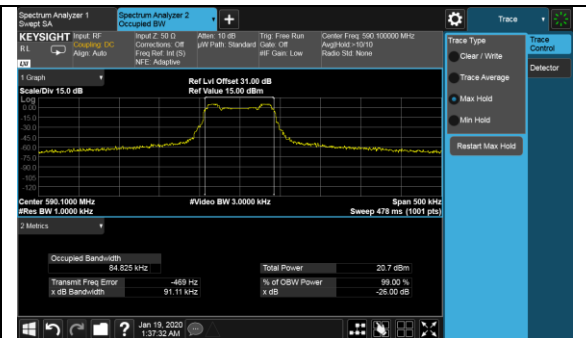
TR-825 HE - Low Channel
