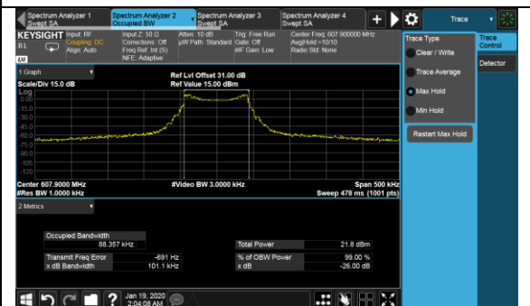
TR-825 HE - High Channel
