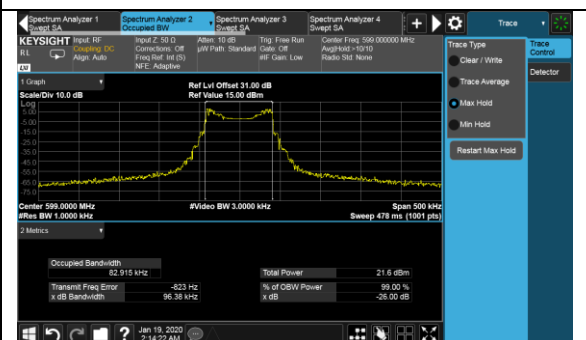
TR-825 HE - Middle Channel
