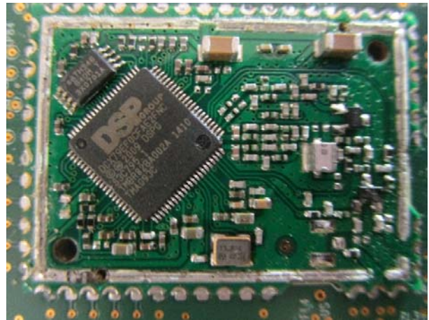
RF Module Cover Off View
