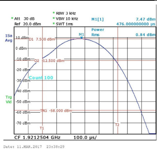
PSD CHAIN 1- Channel 4
