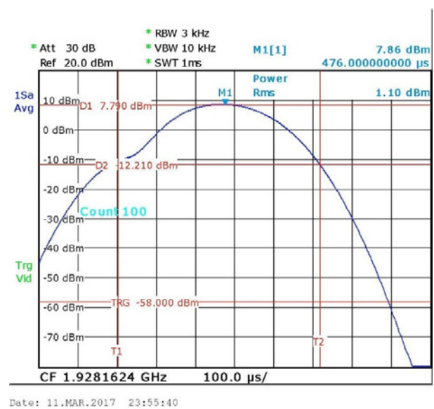
PSD CHAIN 1- Channel 0
