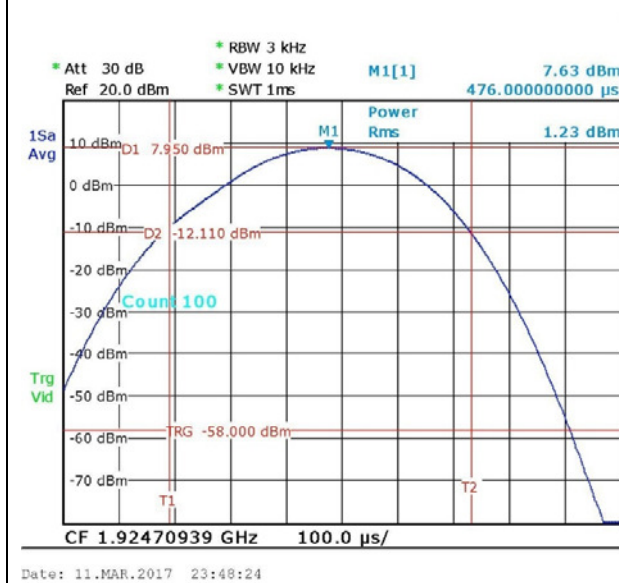
PSD CHAIN 1- Channel 2
