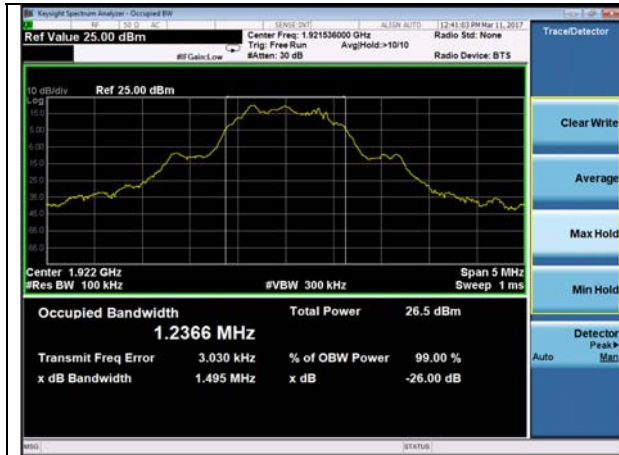
99%OBW -26dB bandwidth-Channel 4
