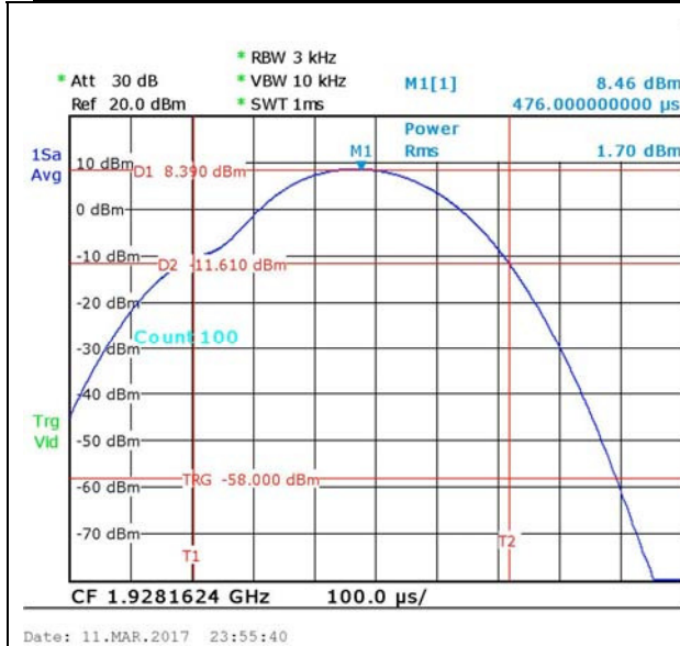
PSD CHAIN 0- Channel 0
