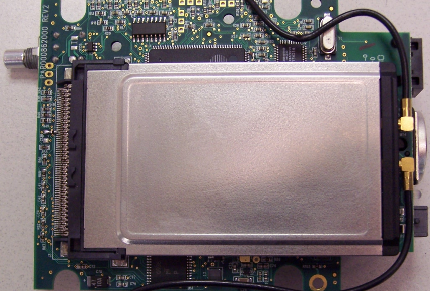
Main PCB with RF Card - Bottom View
