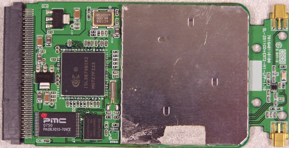
RF Card - Top with Internal Shield View
