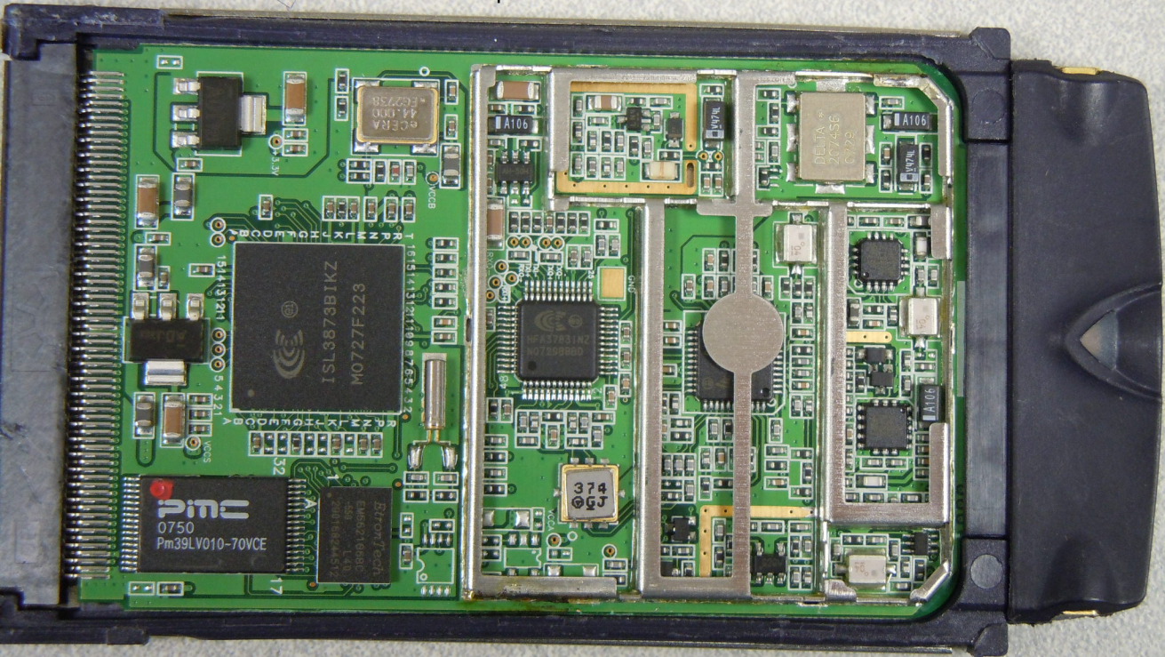
RF Card - Top without Internal Shield View
