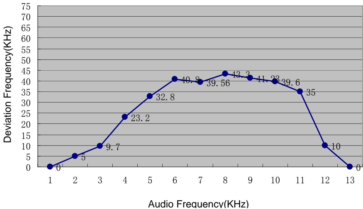
Frequency Response
