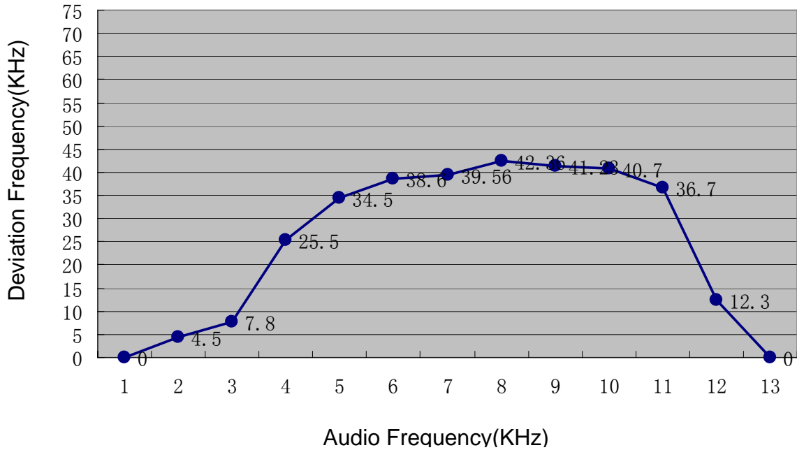
Frequency Response
