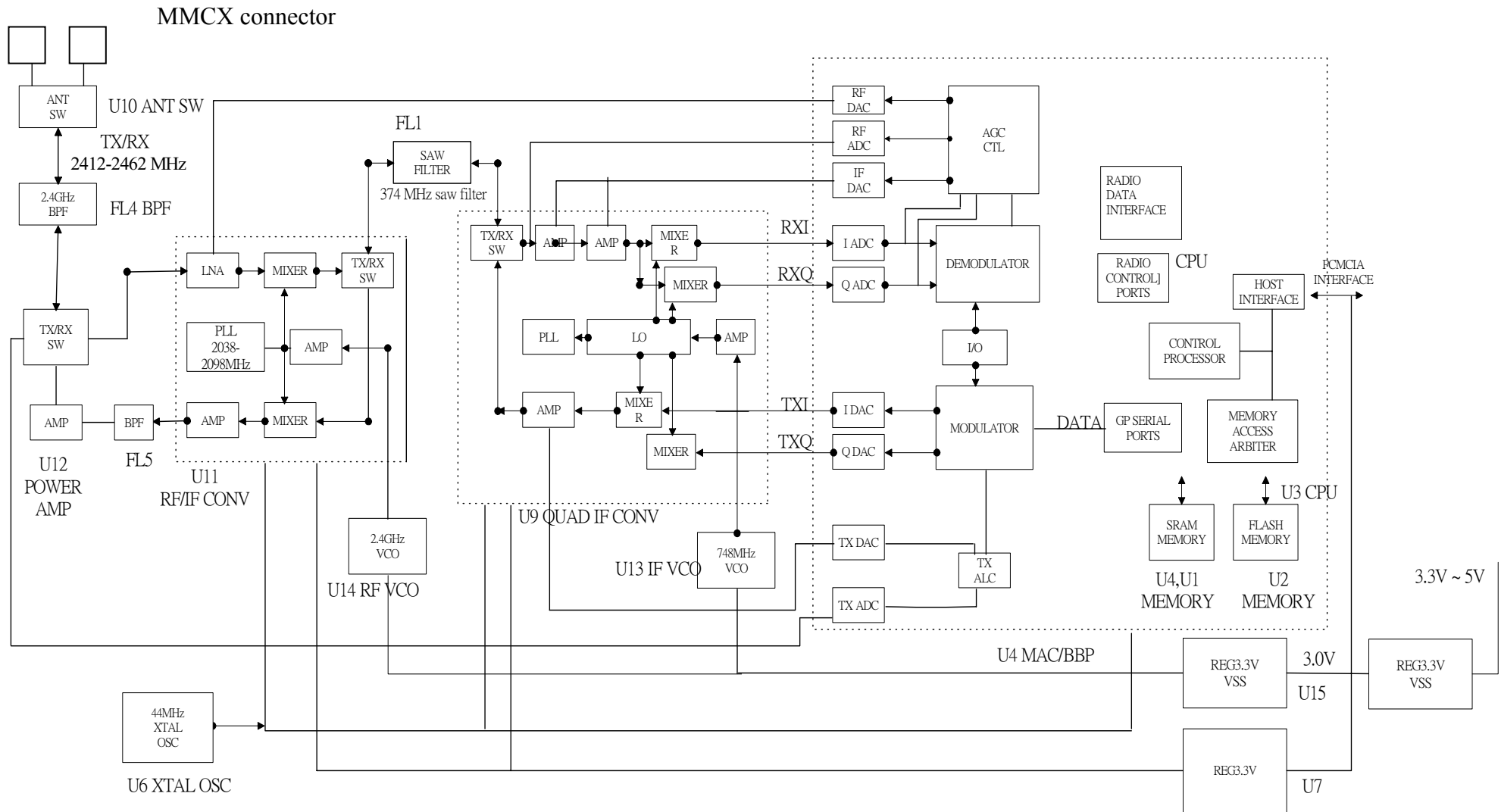
WL-316C WLAN CARD BLOCKDIAGRAM
