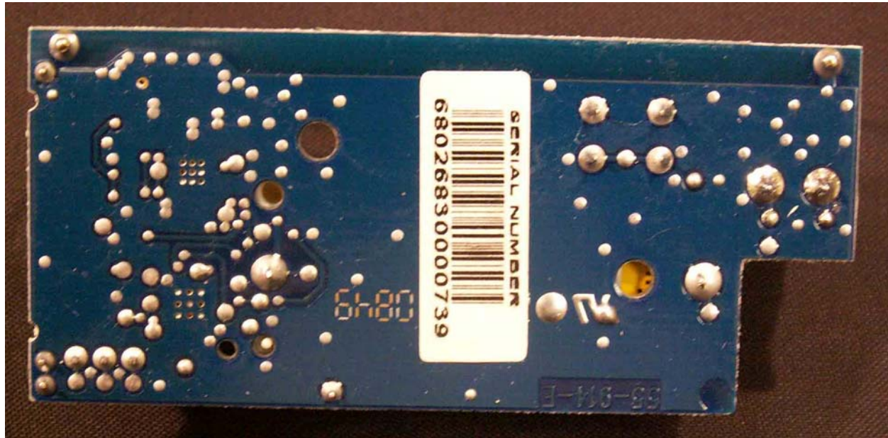
GE Security Inc 319.5MHz Door Window sensor BACK BOARD
