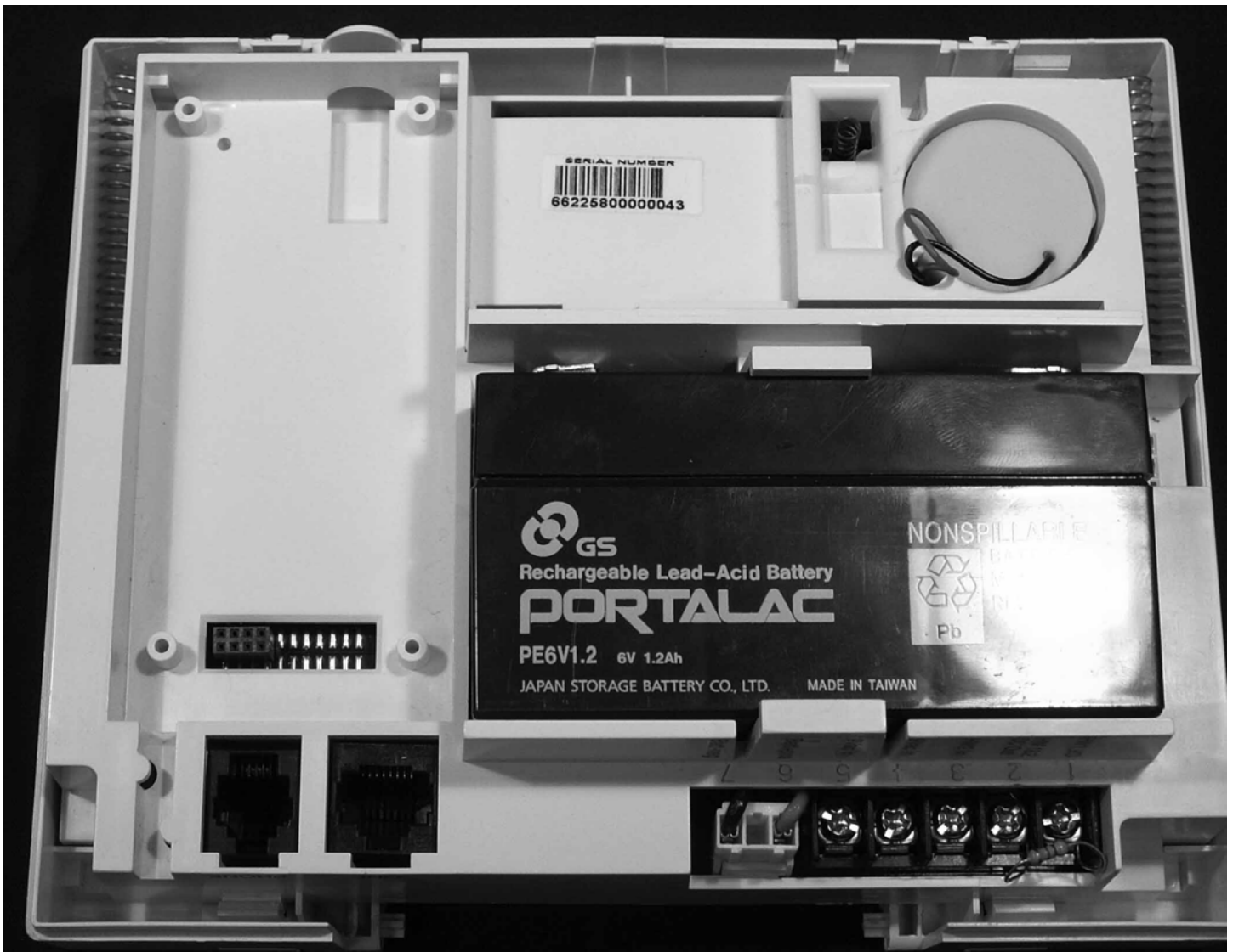
Simon XT Back – Open
