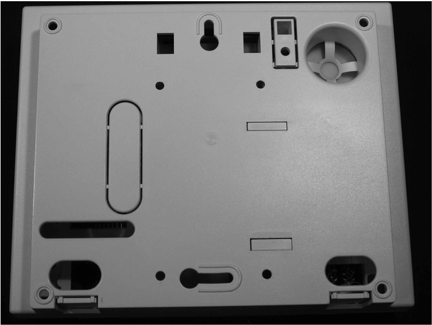
Simon XT Back
