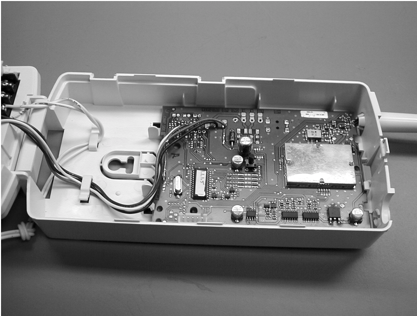
Figure 1: Picture of DUT board inside enclosure.
