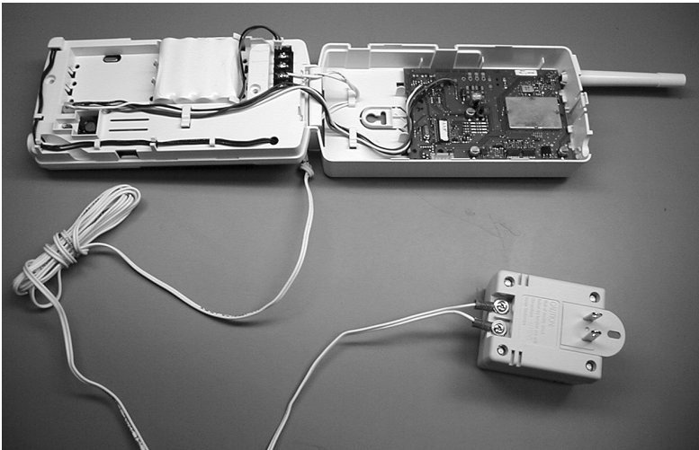
Figure 2: Picture of DUT, showing connection to alarm panel board, antenna shroud, and Class 2 transformer.
