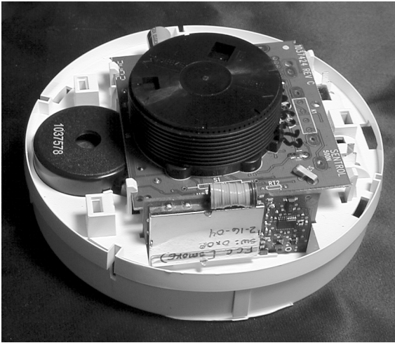
Figure 1: Picture of DUT, showing transmitter board plugged on the motherboard.
