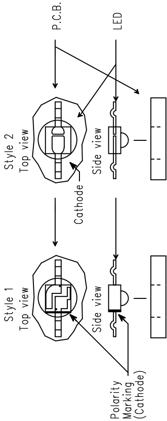
LED insertion detail
