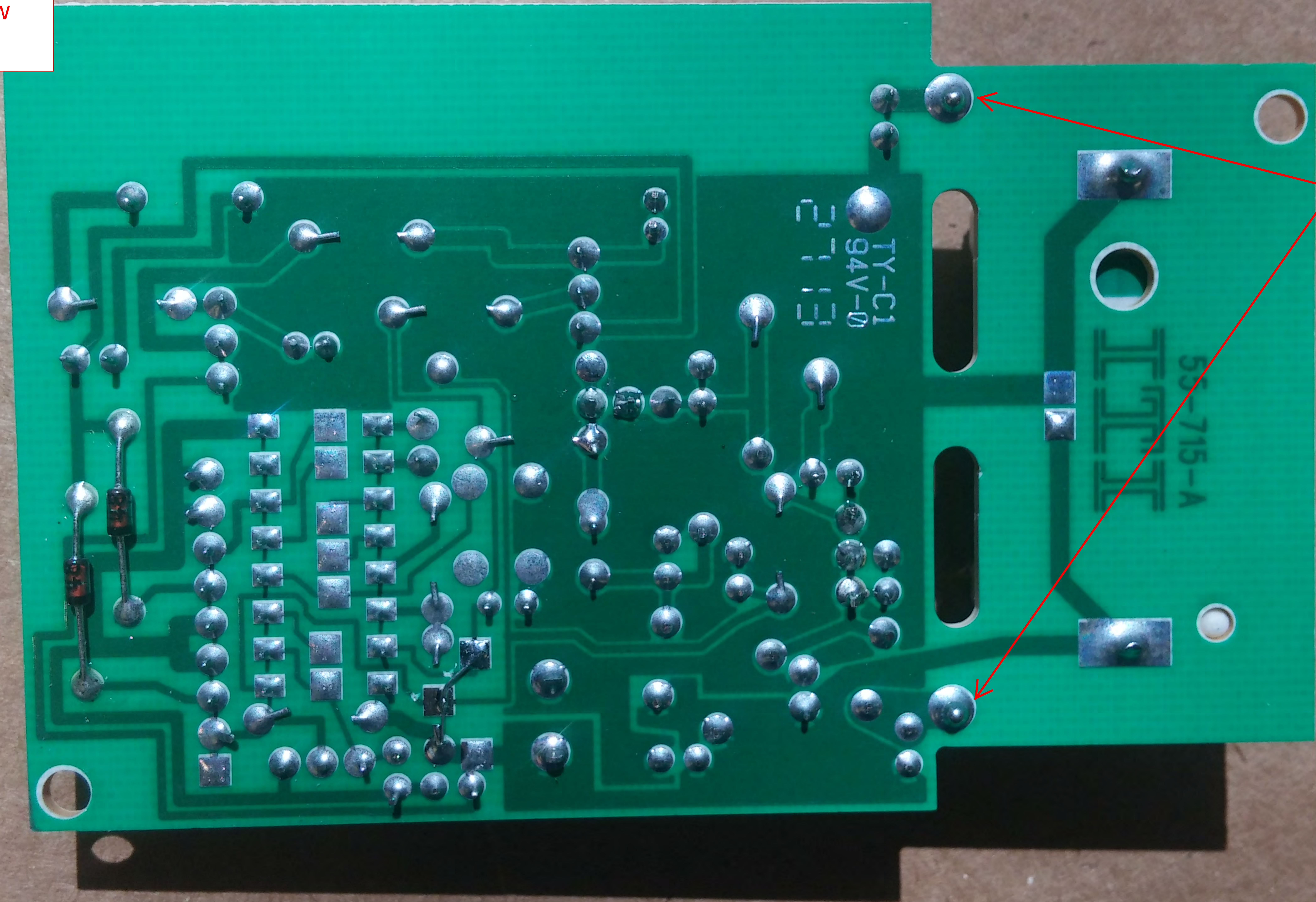
Antenna connections
