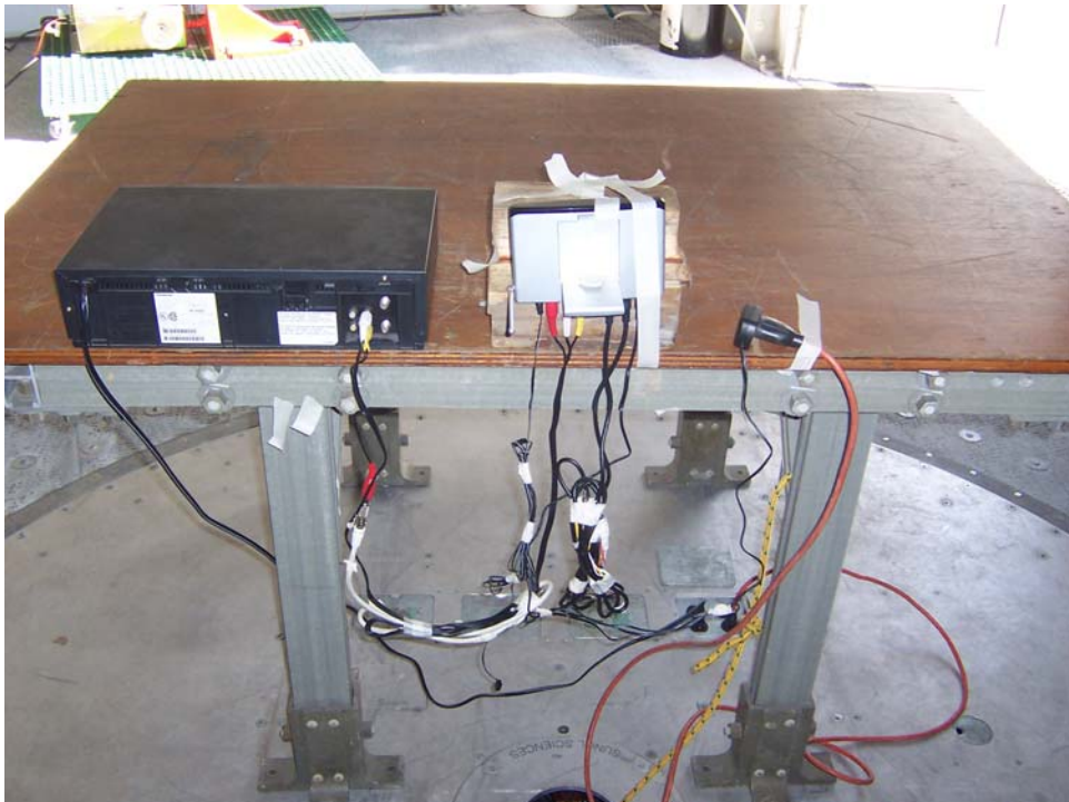
Transmitter, Radiated Emissions, Fundamental and Harmonics, Z-Axis Setup
