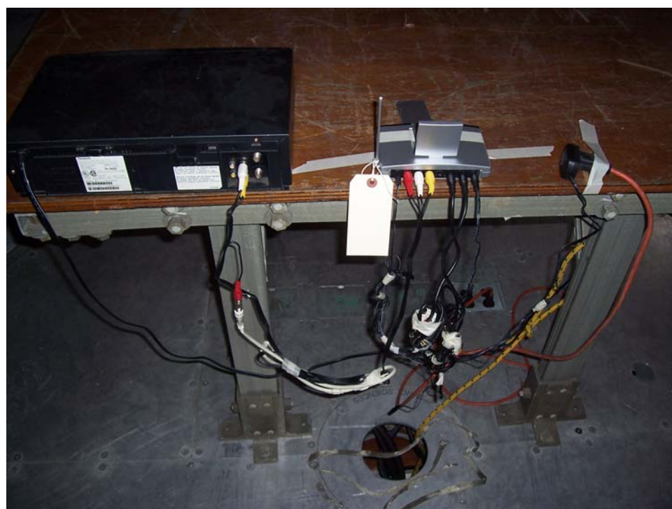
Transmitter, Radiated Emissions, Spurious Case, Rear View Setup
