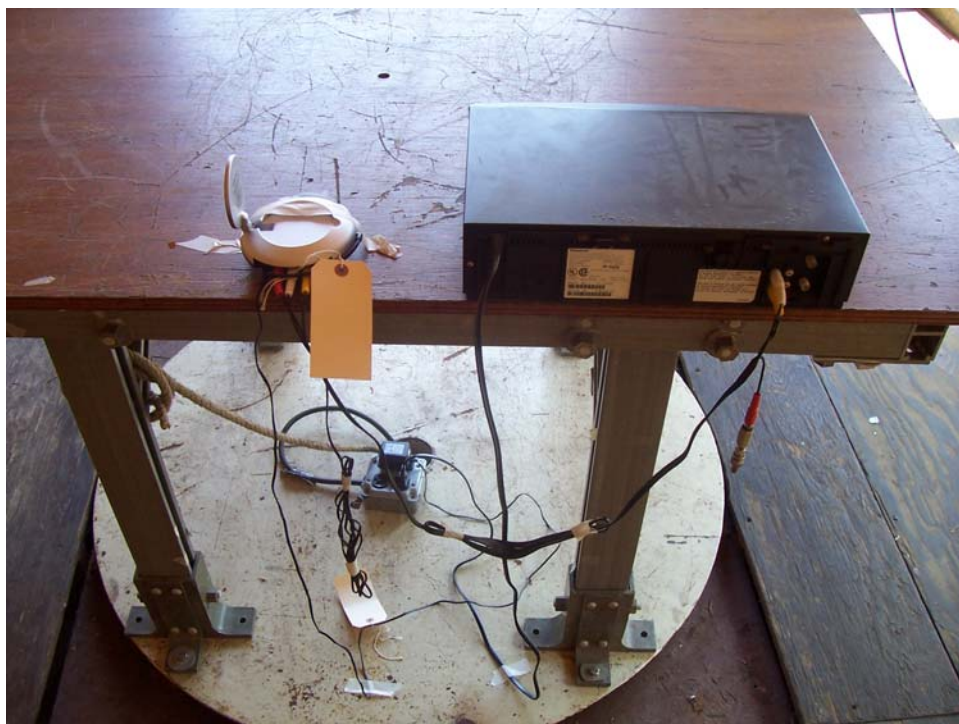
Radiated Emissions, Rear Test Setup
