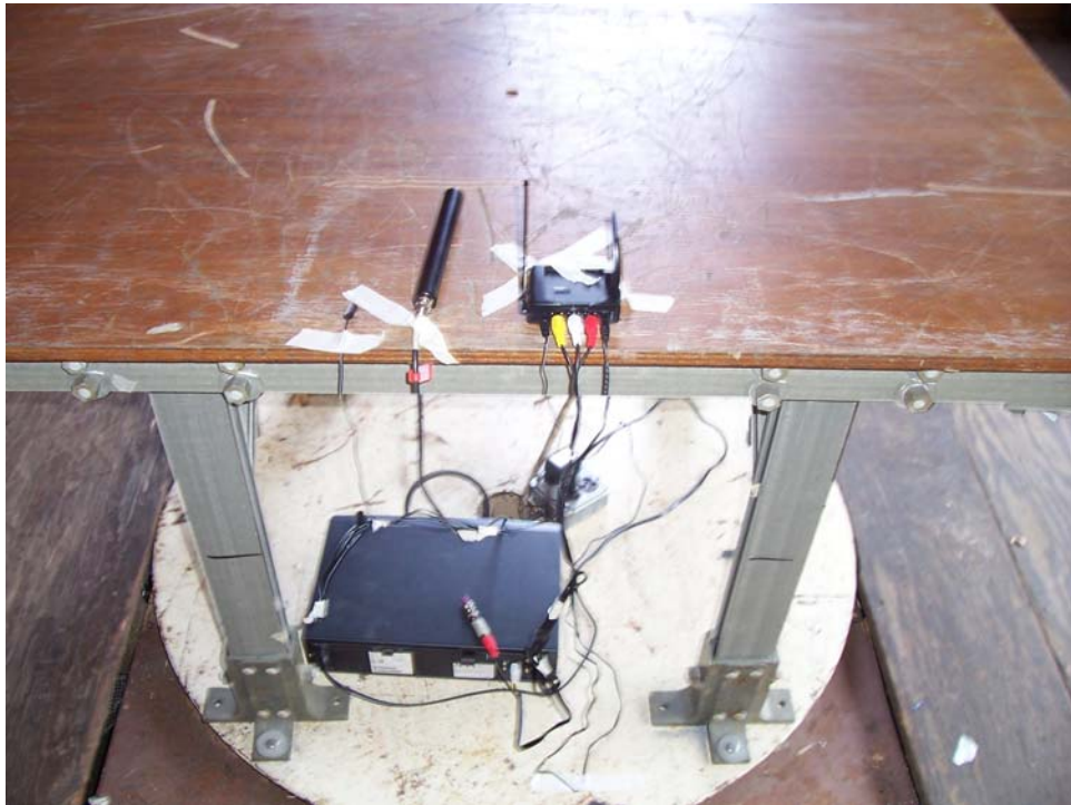
Radiated Emissions, Receiver Test Setup
