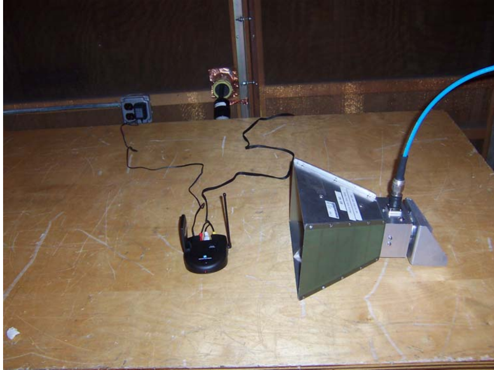
Occupied Bandwidth, Transmitter Test Setup
