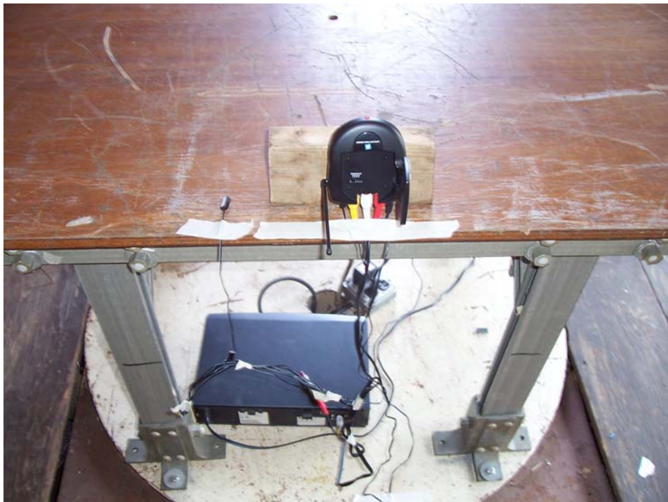
Radiated Emissions, Z-Axis, Transmitter Test Setup
