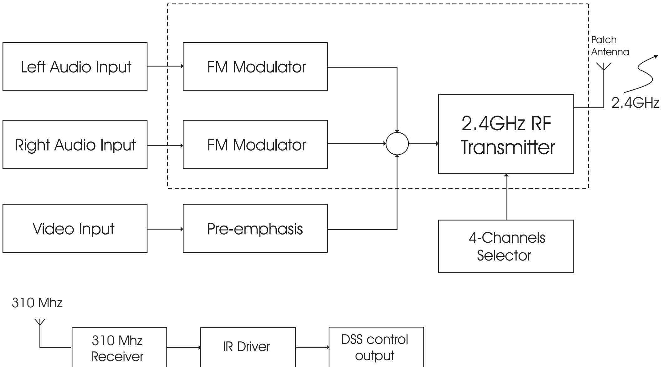
Block Diagram for Video Sender Transmitter VT44A
