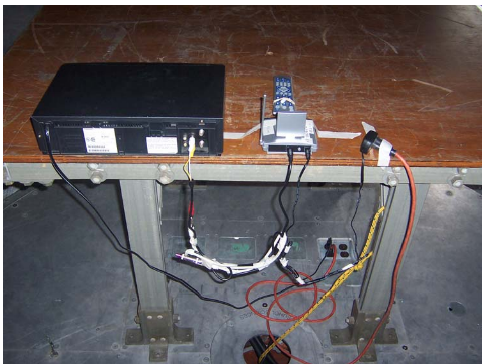
Radiated Emissions, Rear View Setup
