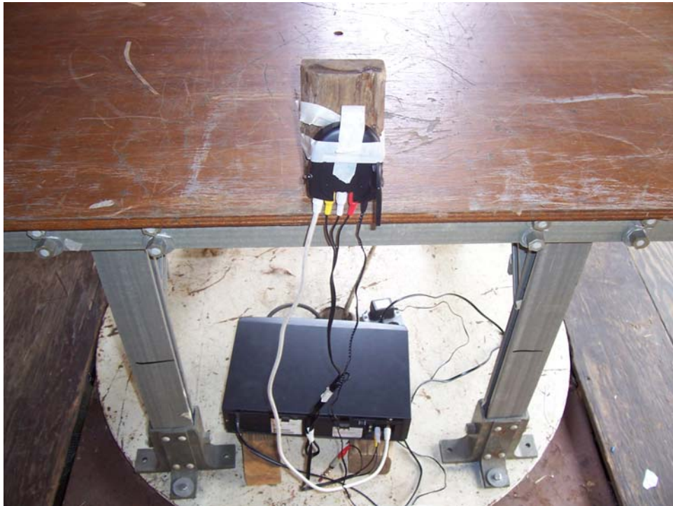
Radiated Emissions, Z-Axis
