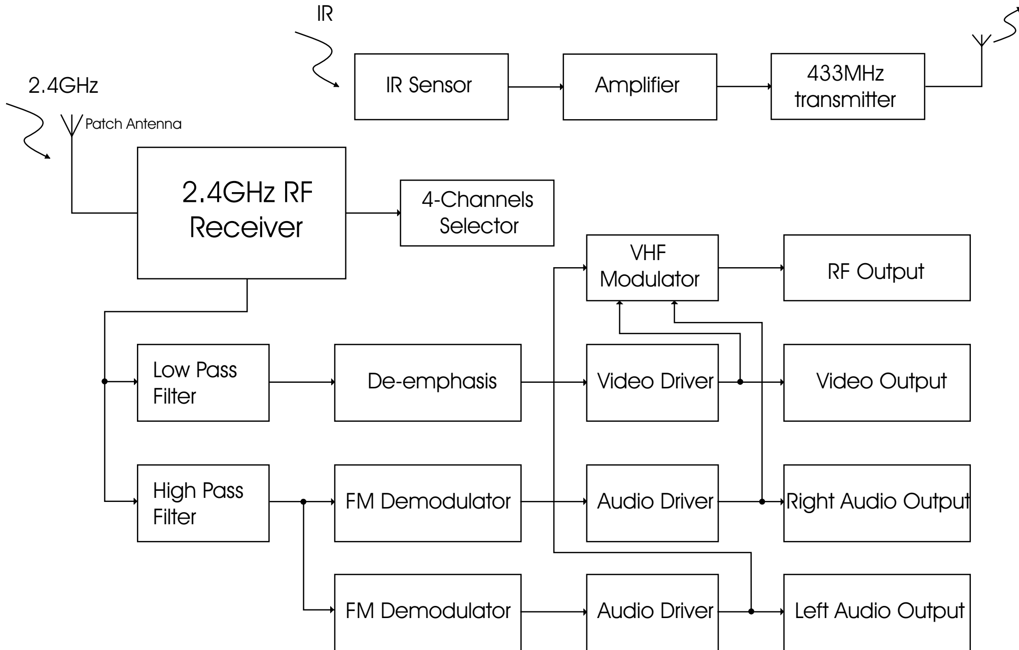
Block Diagram for Video Sender Receiver (VR40A)
