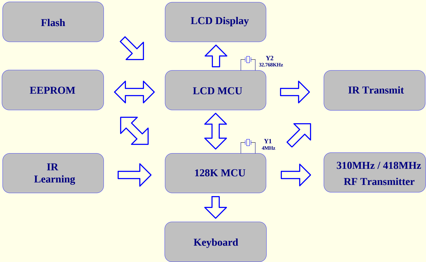
BLOCK DIAGRAM OF IR34A Icon Remote
