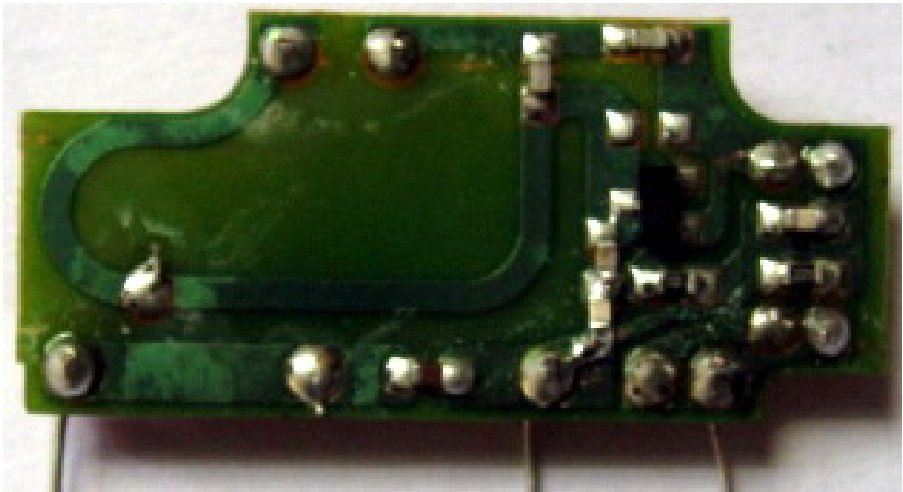
310 MHz, Bottom View
