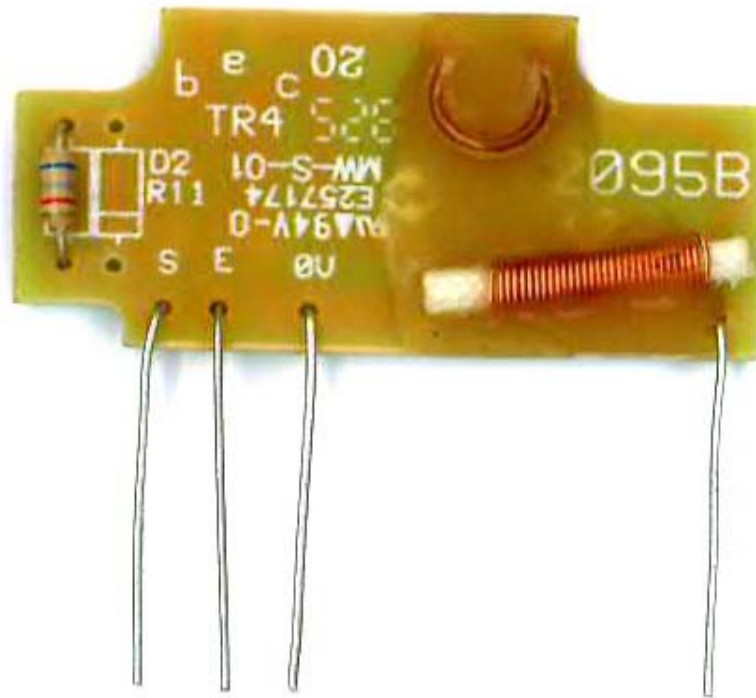
418 MHz, Top View
