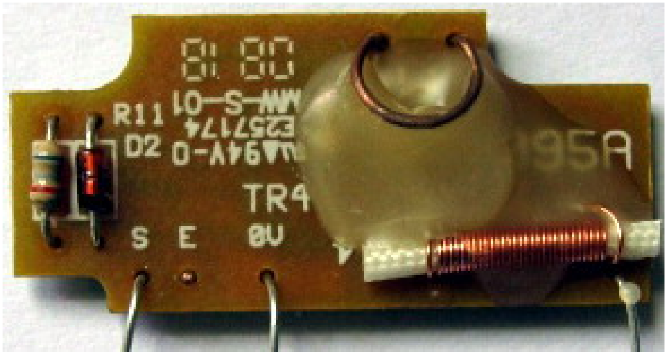
310 MHz, Top View
