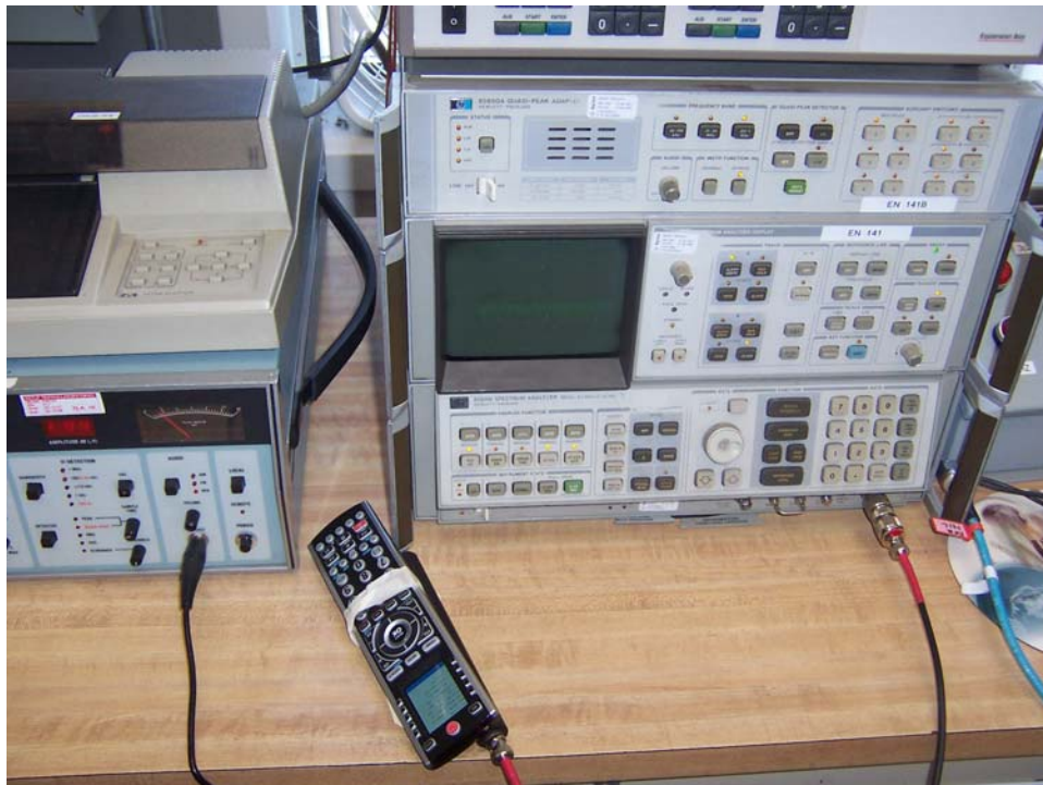
Duty Cycle Determination and Occupied BW, Test Setup
