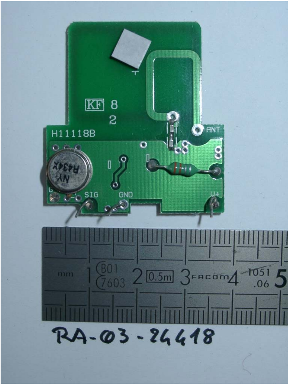
Module radio transmitter: face 1
