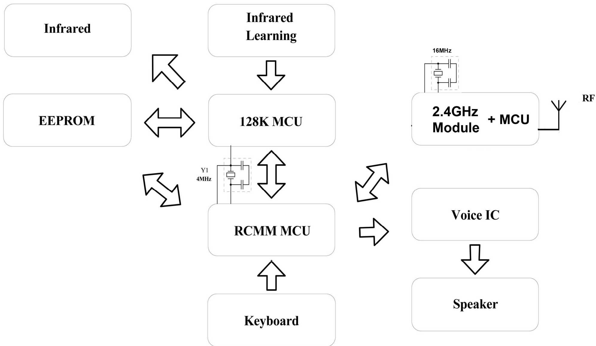
Block Diagram of MXV3RF Remote Control
