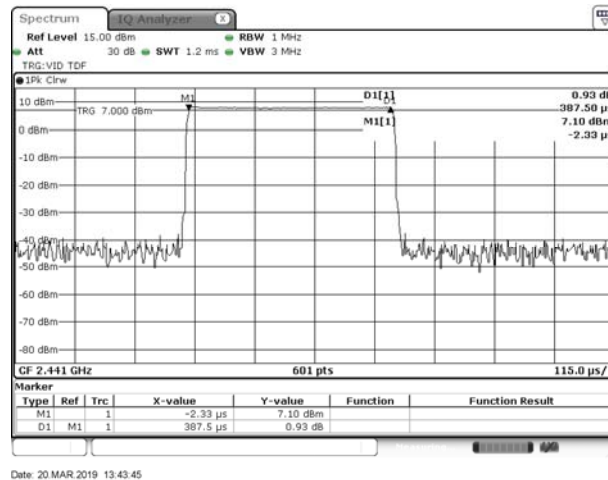
GFSK DH1
