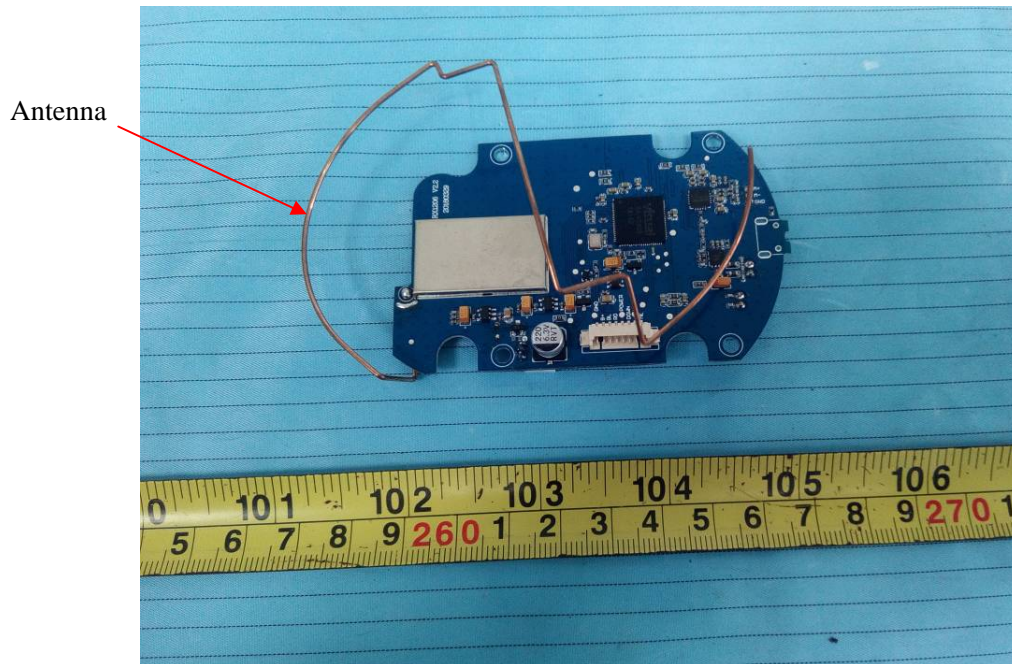
EUT – Mainboard 1 Top View
