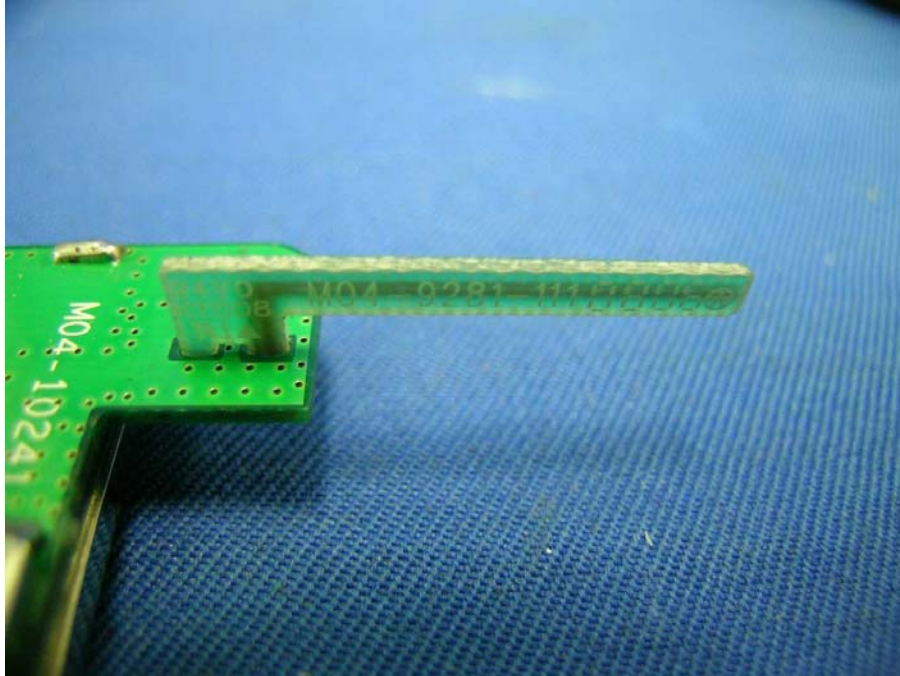
Master Unit TX Antenna PCB rear side
