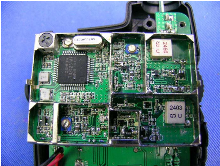
Master Unit Oscillator PCB comp side
