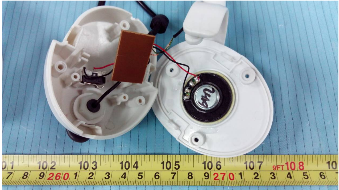
EUT (Headset 1) – Main Board Bottom View
