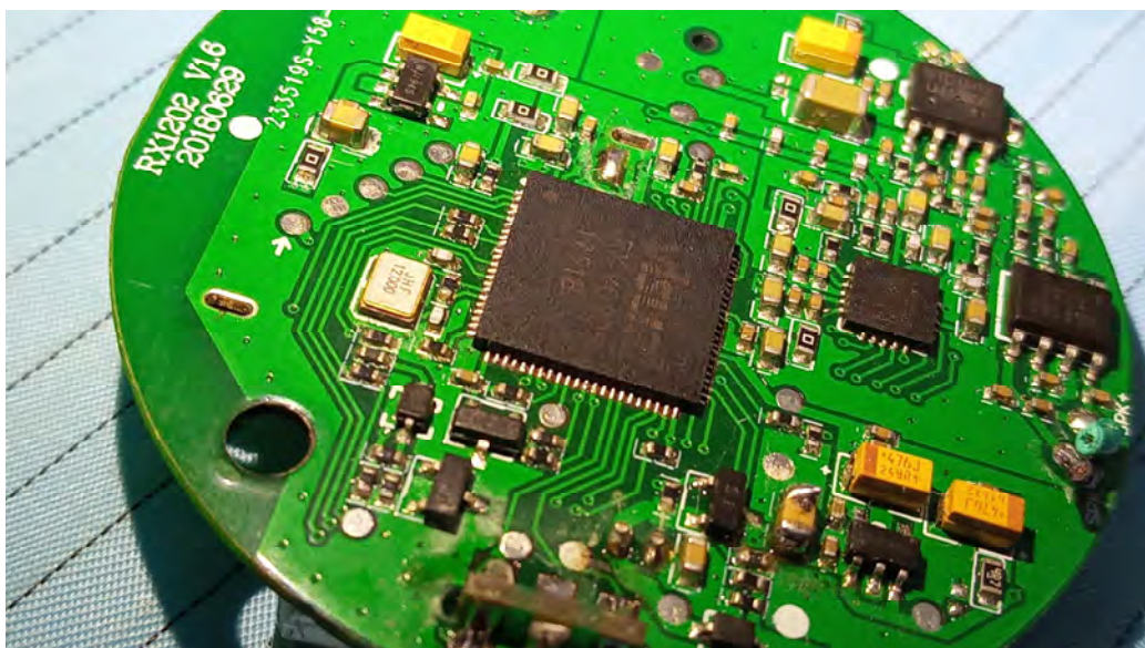
EUT – Main Chip View 1
