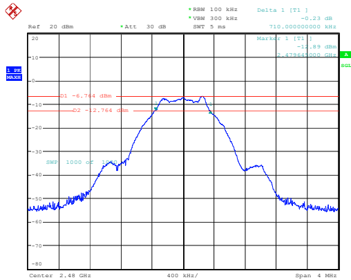
High Channel 0.710MHz
