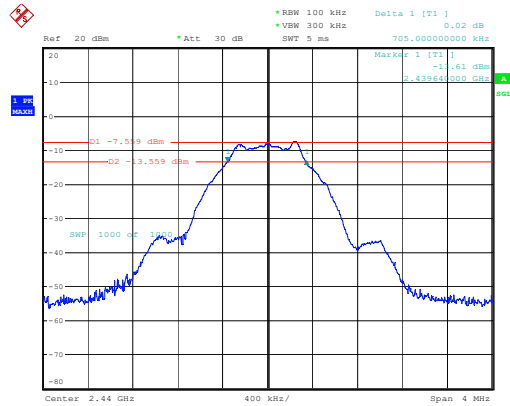
Middle Channel 0.705MHz
