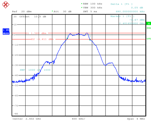
Low Channel 0.680MHz
