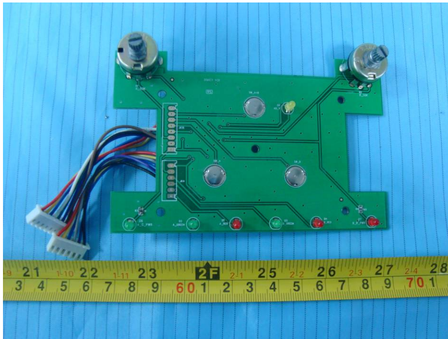
EUT – Button & Indicator Board Bottom View
