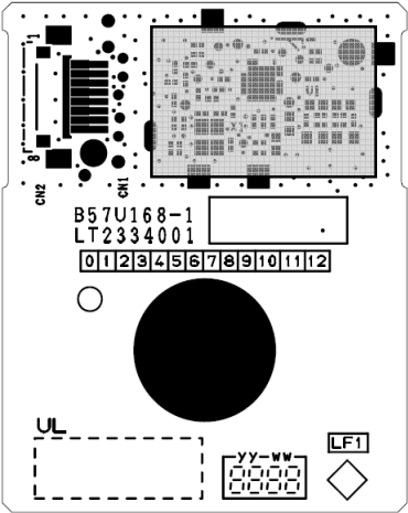
Component Side View
