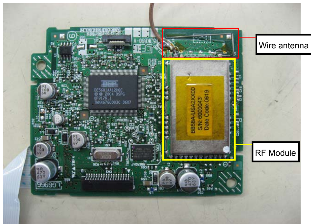
Wire antenna
