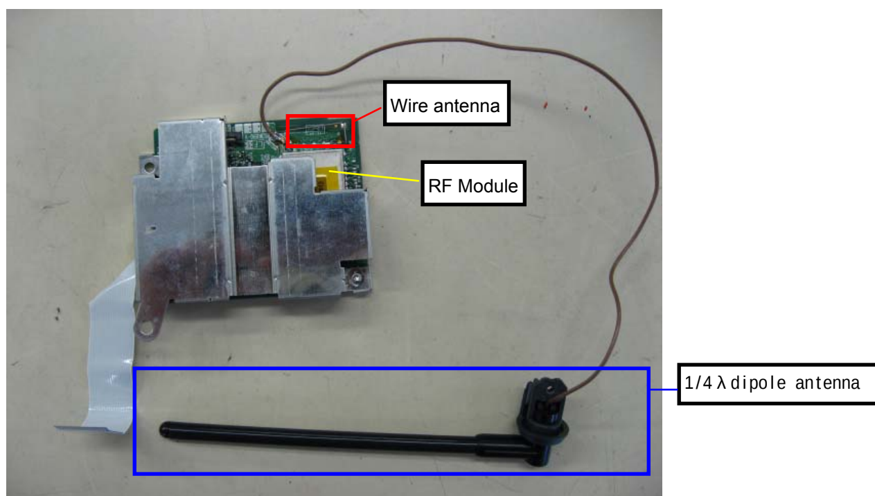
1/4λdipole antenna
