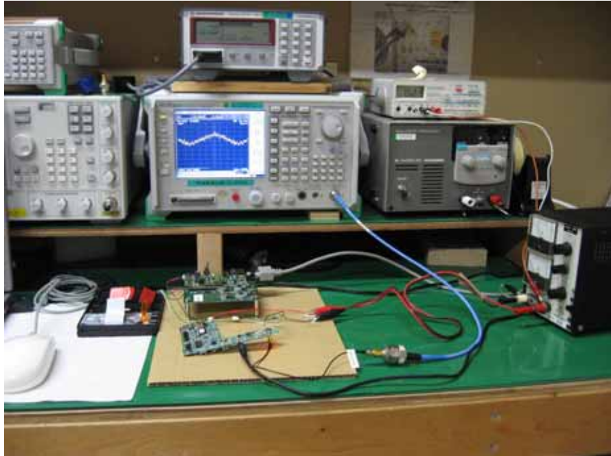
Setup Photo (All Other Test Items)
