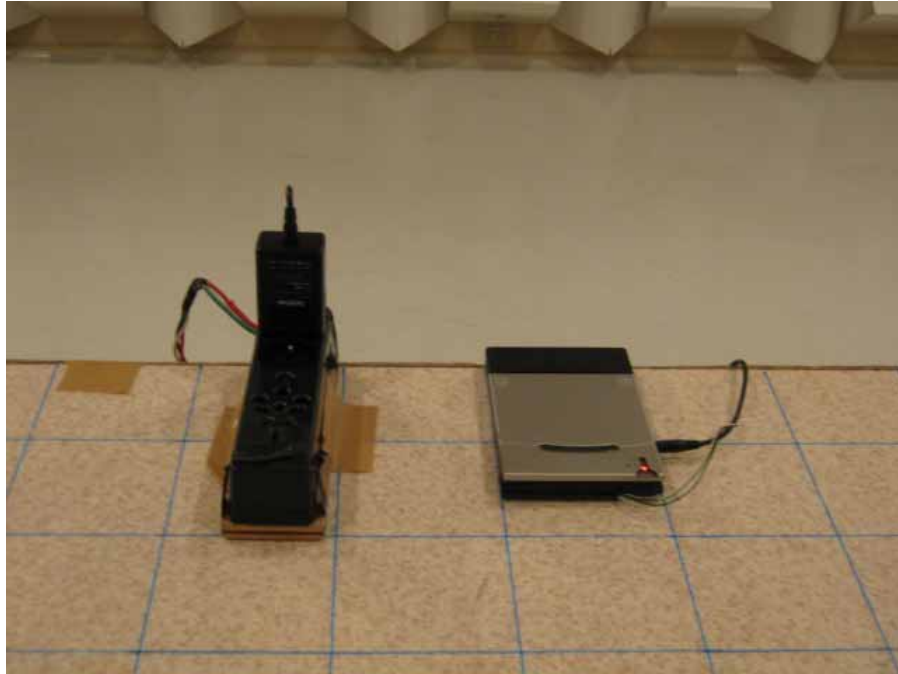
Setup Photo (Radiated Emission)
