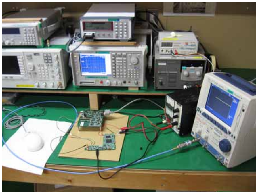
Setup Photo (Maximum Peak Output Power)
