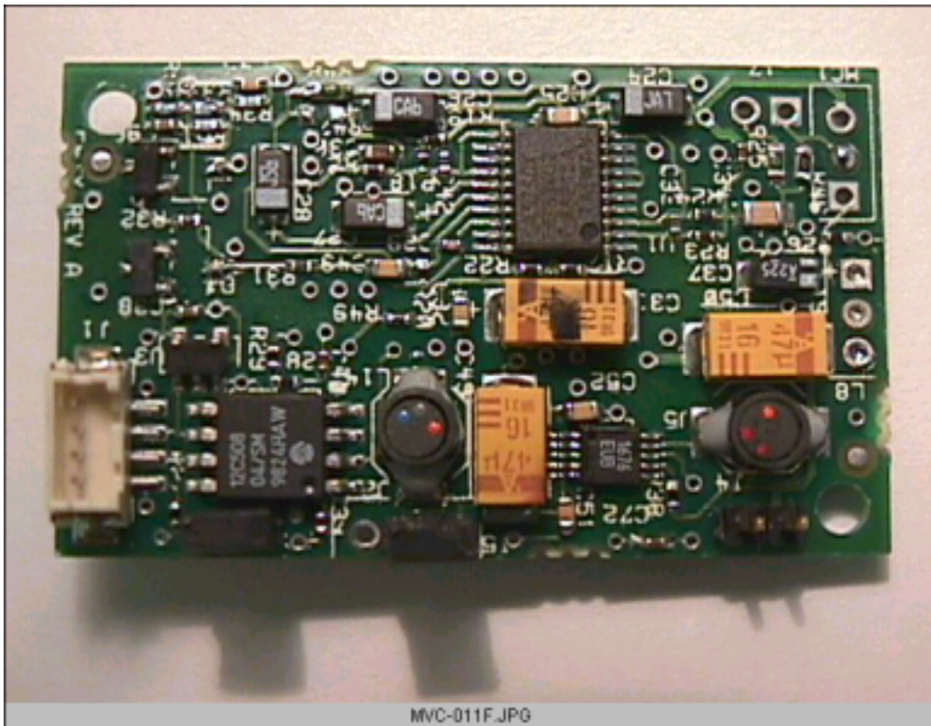
AID - PCB showing Audio and Microprocessor side
