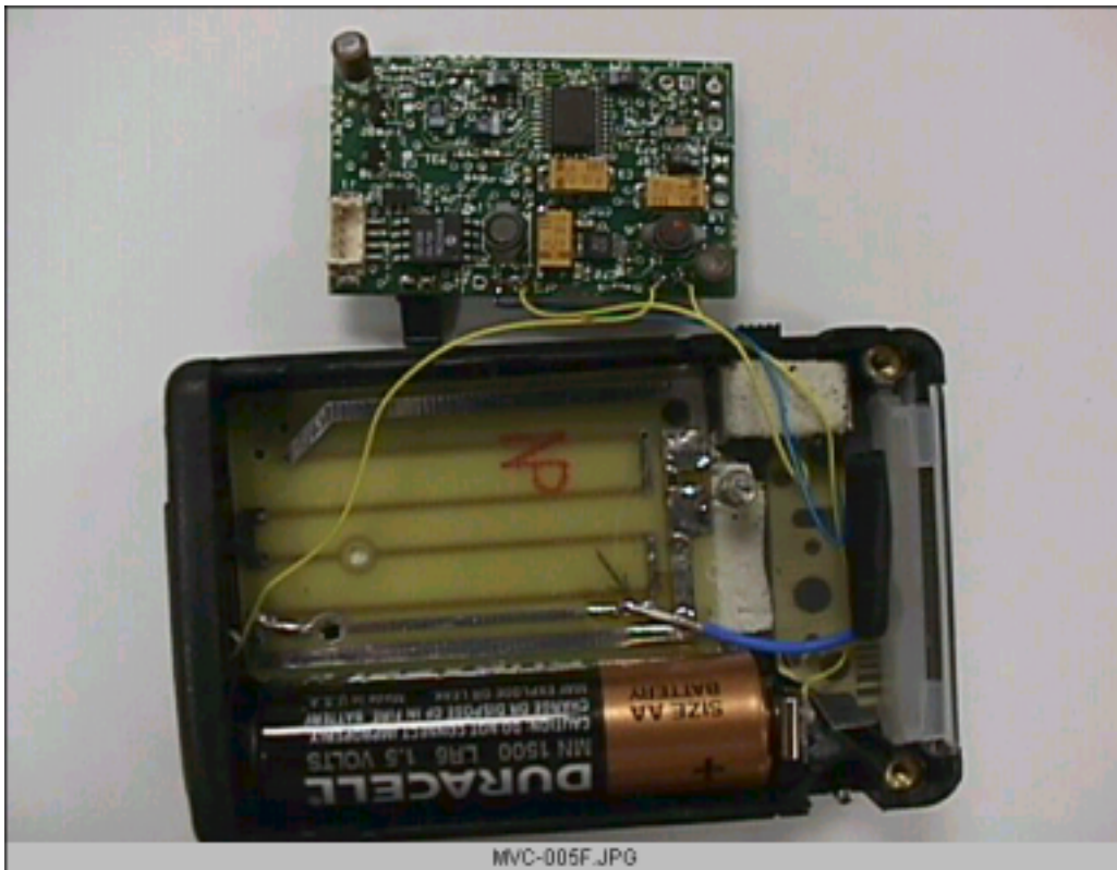
AID - FM Transmitter out of Case showing connections, Audio and Microprocessor PCB side and Antenna Board.
