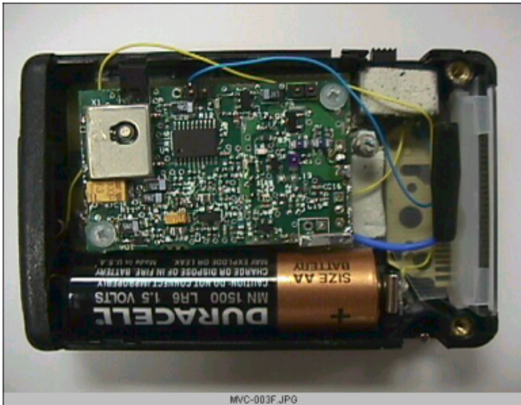
AID - PCB Component Side within case showing RF side
