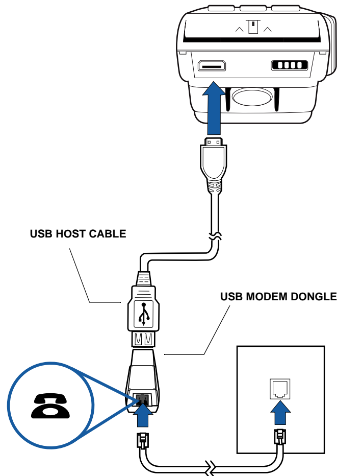
Figure 8 VX 680 USB Modem Dongle Connection
