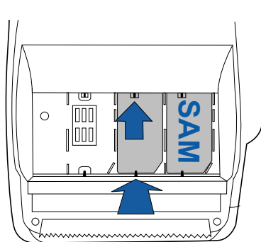
Figure 18 Installing MSAM Card
