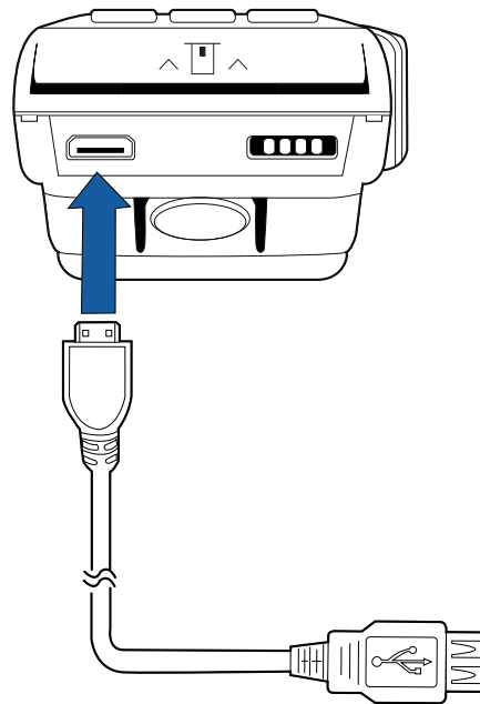
Figure 5 USB Host Cable Connection to a VX 680 Terminal
