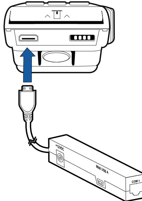
Figure 6 Multi-port Adapter Connection to a VX 680 Terminal
