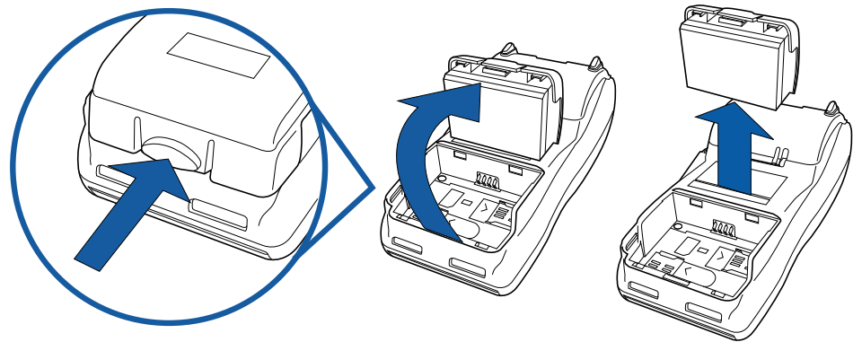
Figure 25 Detaching the Smart Battery from the VX 680 Terminal
