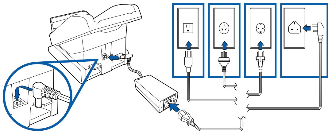
Figure 30 Connecting the Base Station to a Power Source
