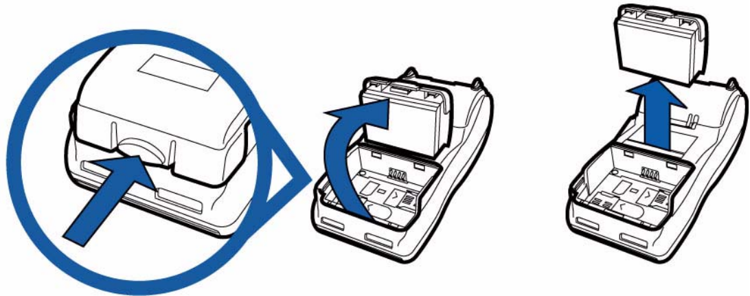
Figure 22 Detaching the Smart Battery from the V×680 Terminal
