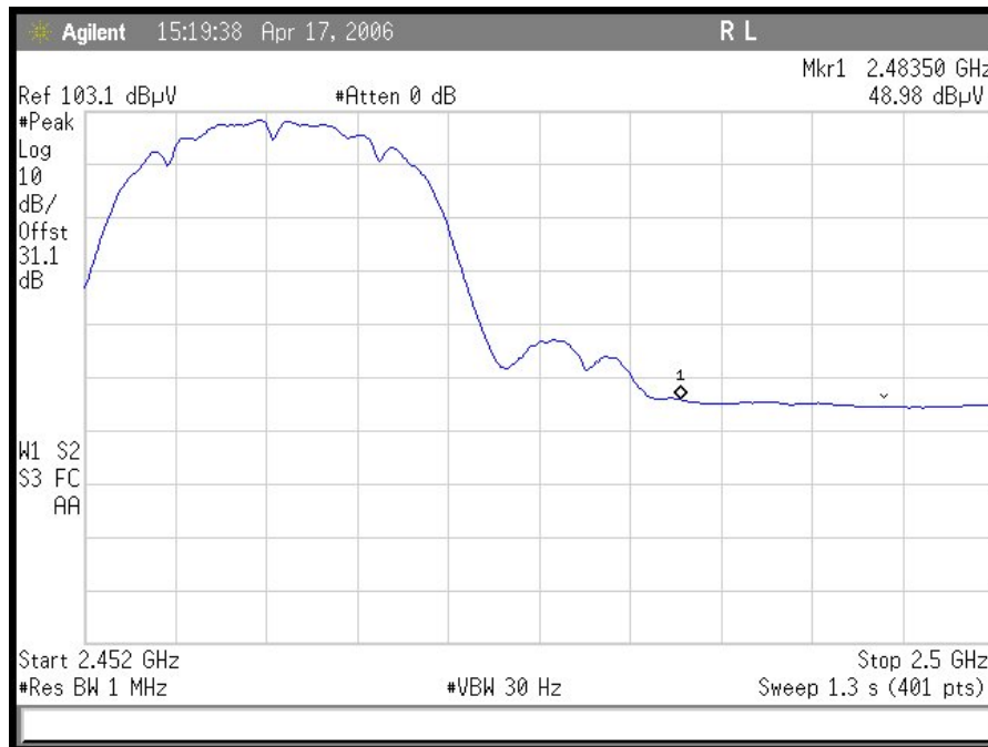
Plot 10. DSSS Radiated Restricted Band 2483.5 MHz – 2500 MHz Average
