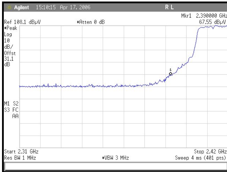
Plot 11. OFDM Radiated Restricted Band 2310 MHz – 2390 MHz Peak
