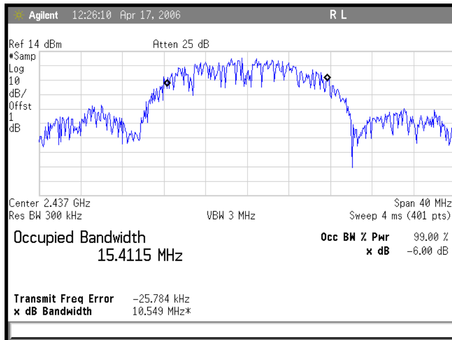
Plot 2. 802.11/g Mid Ch DSSS Occupied Band Width
