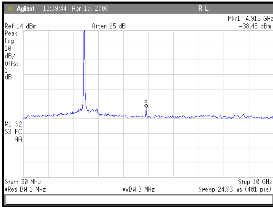
Plot 23. 802.11/g – High Channel DSSS Conducted Emissions 30MHz - 10GHz
