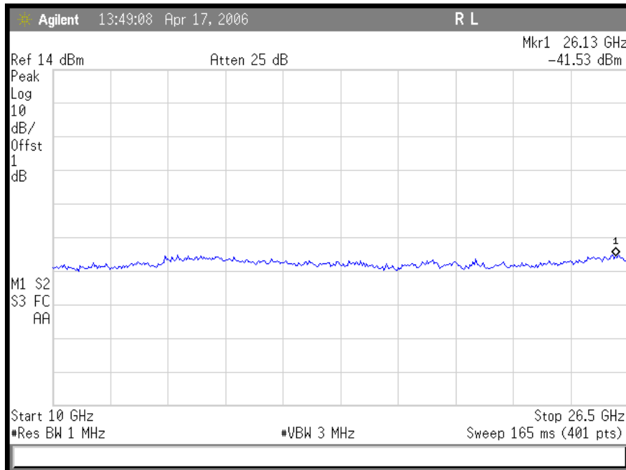
Plot 22. 802.11/g – Mid Channel OFDM Conducted Emissions 10 – 26.5GHz
