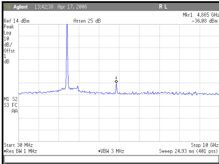
Plot 20. 802.11/g – Mid Channel OFDM Conducted Emissions 30MHz - 10GHz
