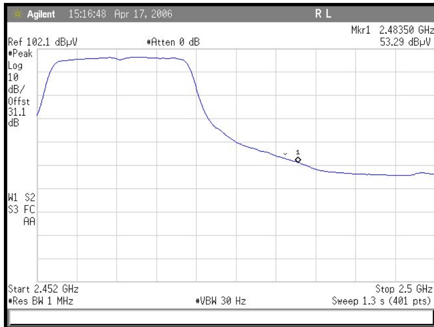
Plot 14. OFDM Radiated Restricted Band 2483.5 MHz – 2500 MHz Average
