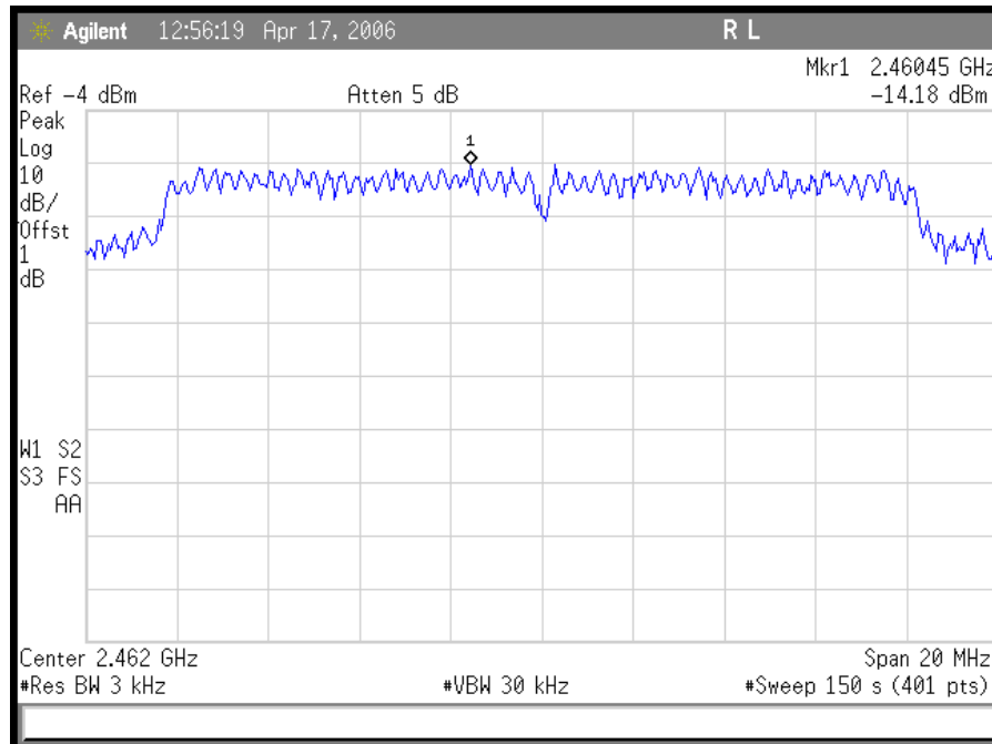
Plot 36. 802.11/g – OFDM High Ch Peak Power Spectral Density
