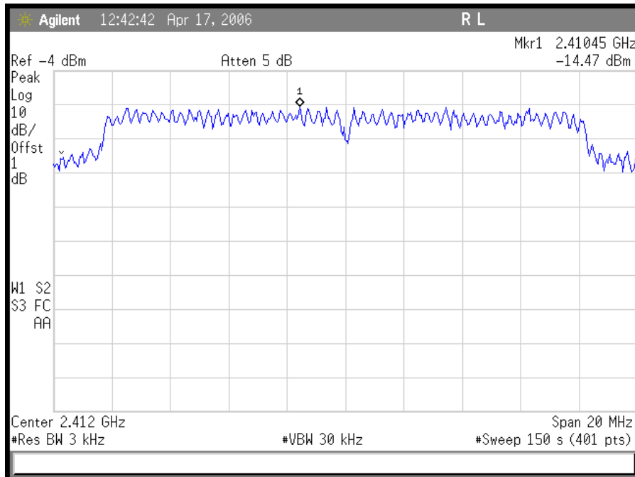
Plot 34. 802.11/g – OFDM Low Ch Peak Power Spectral Density
