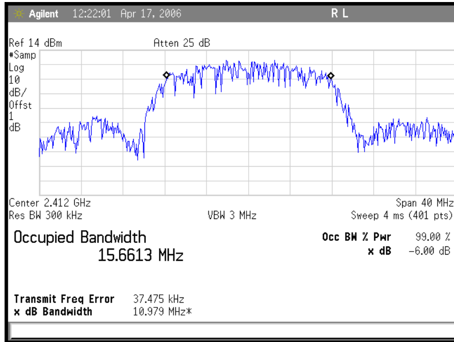
Plot 1. 802.11/g Low Ch DSSS Occupied Band Width
