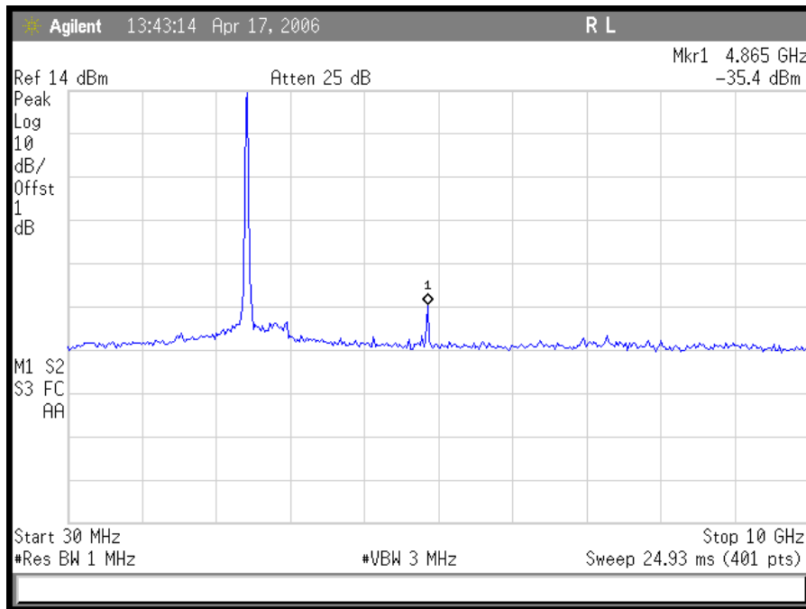
Plot 19. 802.11/g – Mid Channel DSSS Conducted Emissions 30MHz - 10GHz
