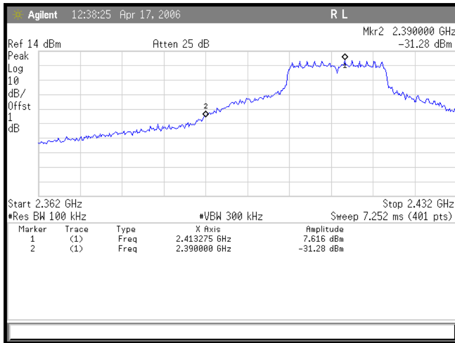
Plot 29. 802.11/g – OFDM Lower Band Edge
