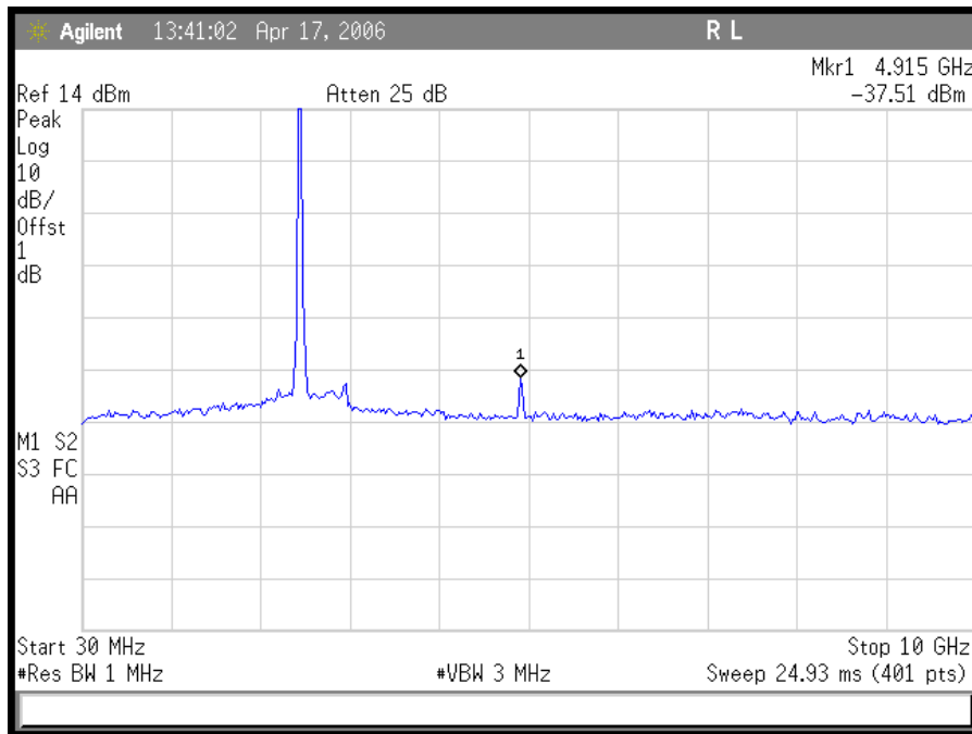
Plot 24. 802.11/g – High Channel OFDM Conducted Emissions 30MHz - 10GHz
