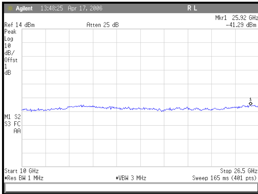
Plot 21. 802.11/g – Mid Channel DSSS Conducted Emissions 10 – 26.5GHz
