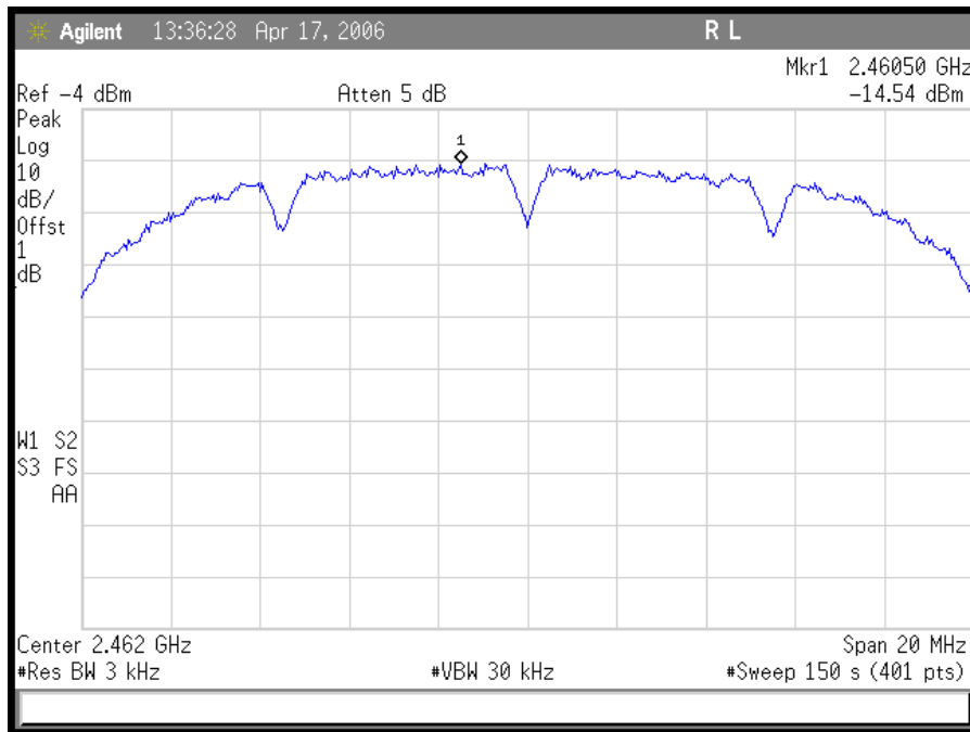
Plot 33. 802.11/g – DSSS High Ch Peak Power Spectral Density
