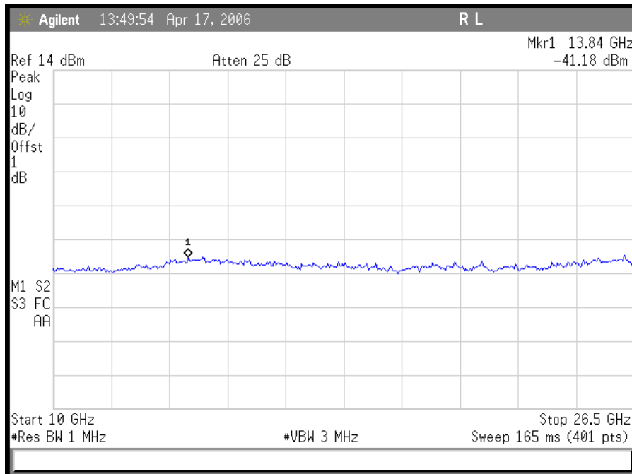
Plot 26. 802.11/g – High Channel OFDM Conducted Emissions 10 – 26.5GHz
