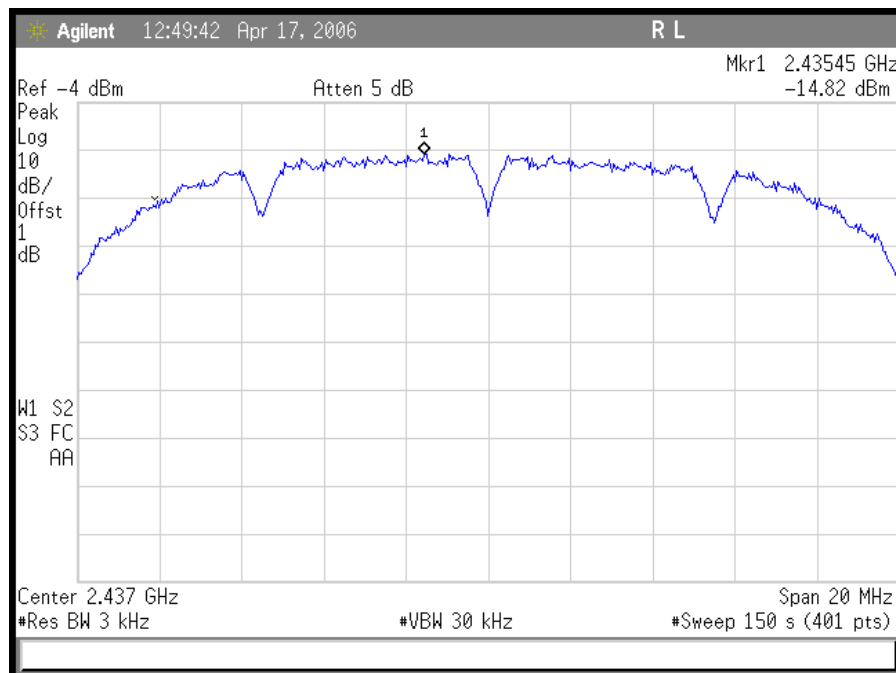
Plot 32. 802.11/g – DSSS Mid Ch Peak Power Spectral Density
