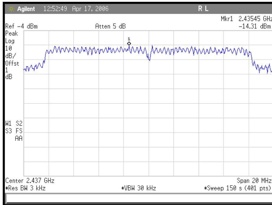
Plot 35. 802.11/g – OFDM Mid Ch Peak Power Spectral Density
