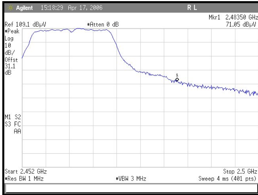
Plot 13. OFDM Radiated Restricted Band 2483.5 MHz – 2500 MHz Peak
