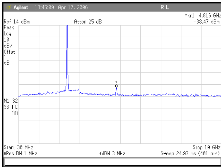
Plot 16. 802.11/g Low Channel OFDM Conducted Emissions 30MHz - 10GHz
