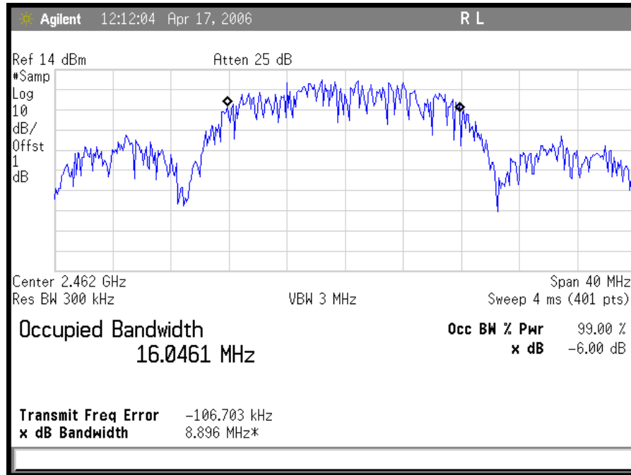
Plot 3. 802.11/g High Ch DSSS Occupied Band Width
