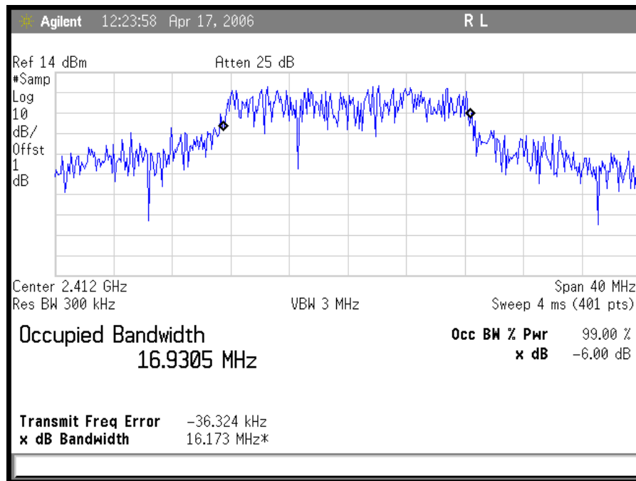
Plot 4. 802.11/g Low Ch OFDM Occupied Band Width
