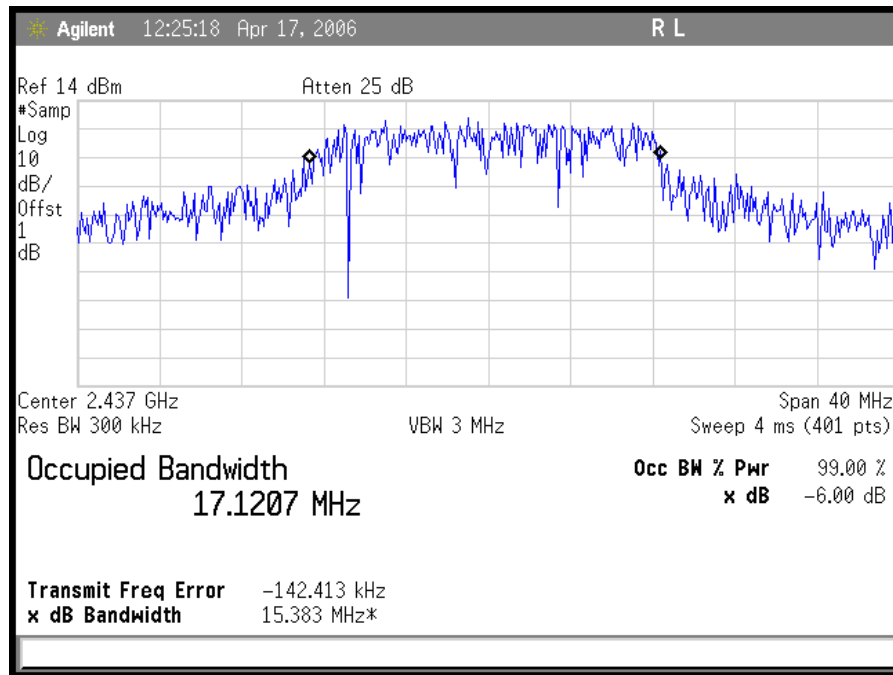
Plot 5. 802.11/g Mid Ch OFDM Occupied Band Width
