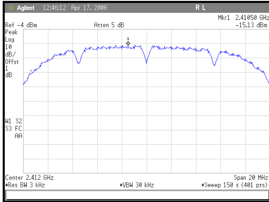
Plot 31. 802.11/g – DSSS Low Ch Peak Power Spectral Density
