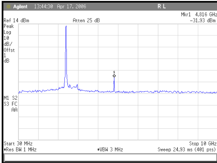
Plot 15. 802.11/g Low Channel DSSS Conducted Emissions 30MHz - 10GHz
