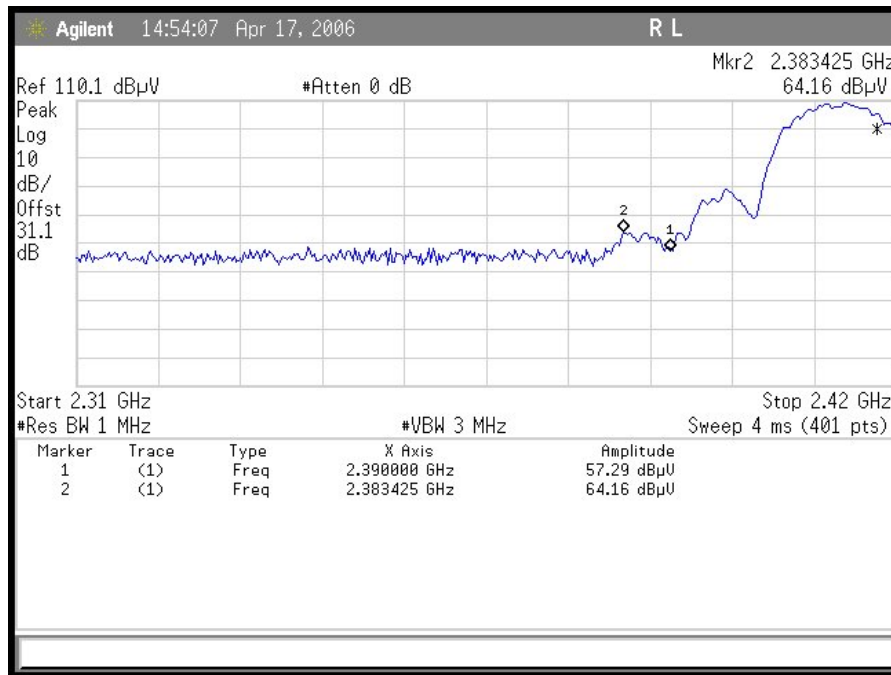
Plot 7. DSSS Radiated Restricted Band 2310 MHz – 2390 MHz Peak
