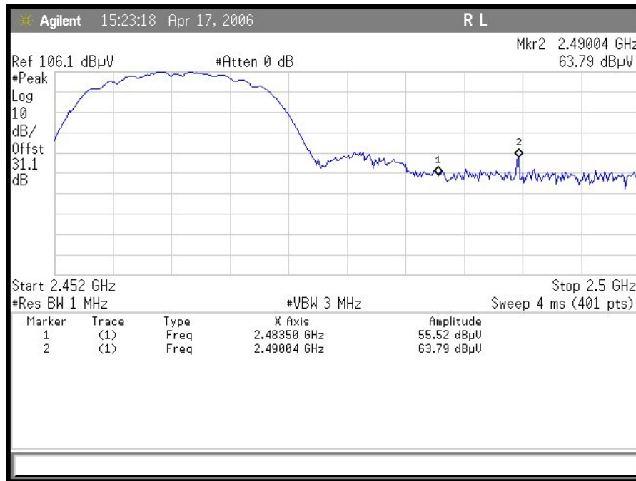
Plot 9. DSSS Radiated Restricted Band 2483.5 MHz – 2500 MHz Peak
