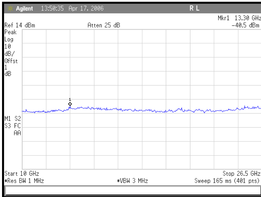
Plot 25. 802.11/g – High Channel DSSS Conducted Emissions 10 – 26.5GHz
