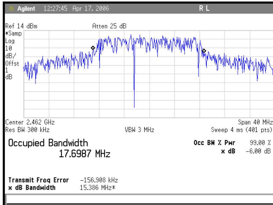
Plot 6. 802.11/g High Ch OFDM Occupied Band Width
