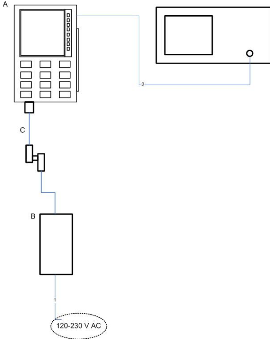
Figure 2. Block Diagram of Test Configuration (Conducted Measurement)
