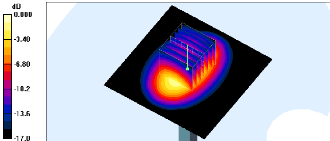
0 dB = 4.89mW/g
