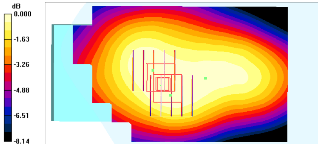
0 dB = 0.218mW/g
