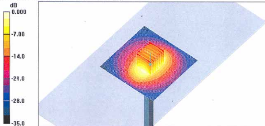
0 dB = 11.6mW/g
