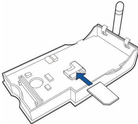
Figure 39 Insert SIM Card Into GSM/GPRS Sled Module
