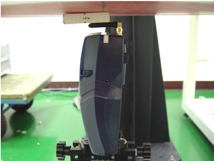
DUT Top Side and Antenna with 1.5cm Gap
