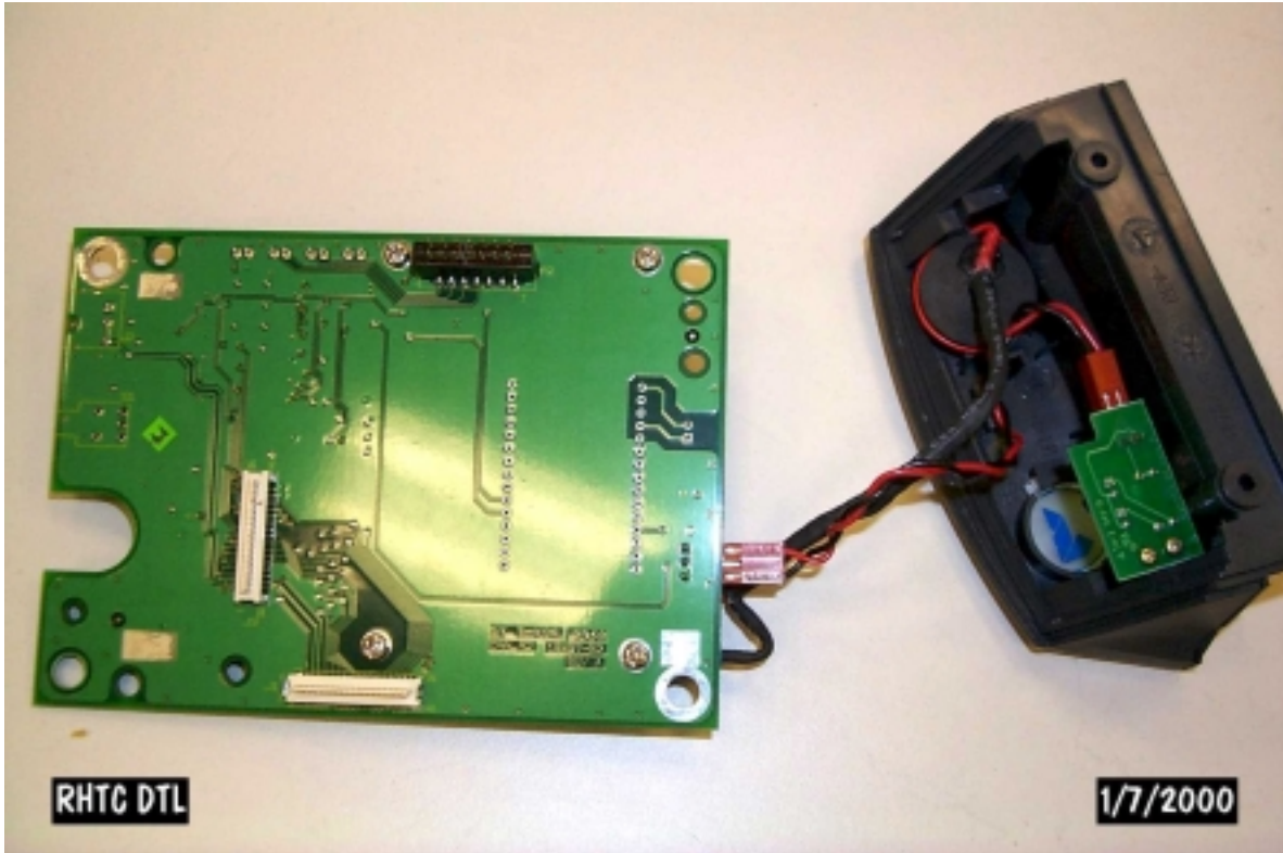
Photo 1 – Main printed circuit board – bottom side
