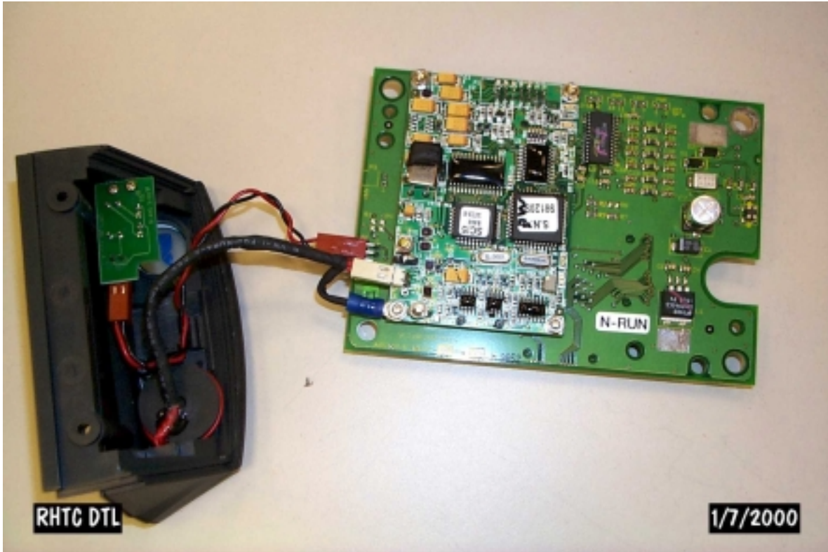
Photo 3 – Main printed circuit board removed from case showing connections to antenna and LED board
