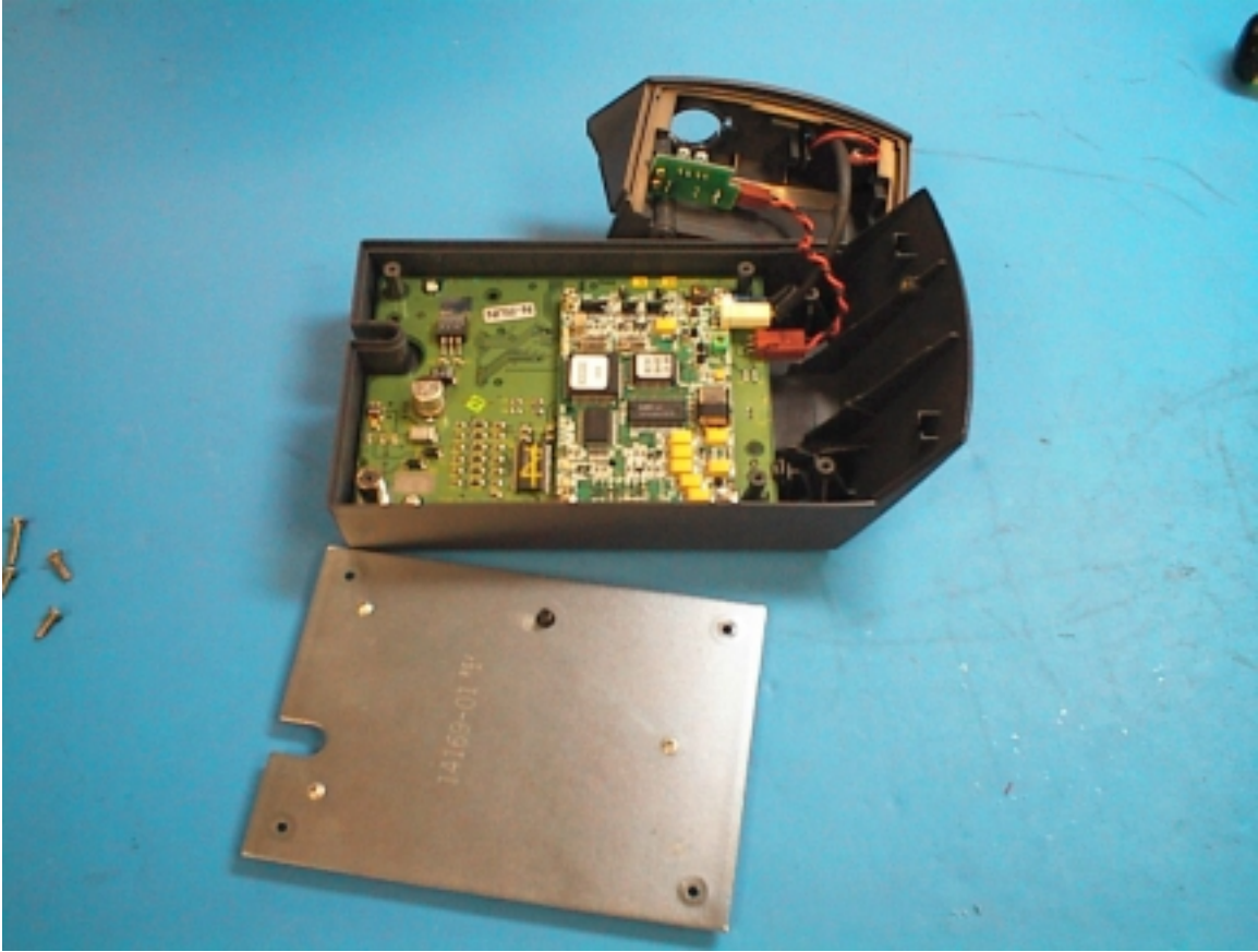
Photo 2 – Disassembled, showing LED PC board and antenna mounting
