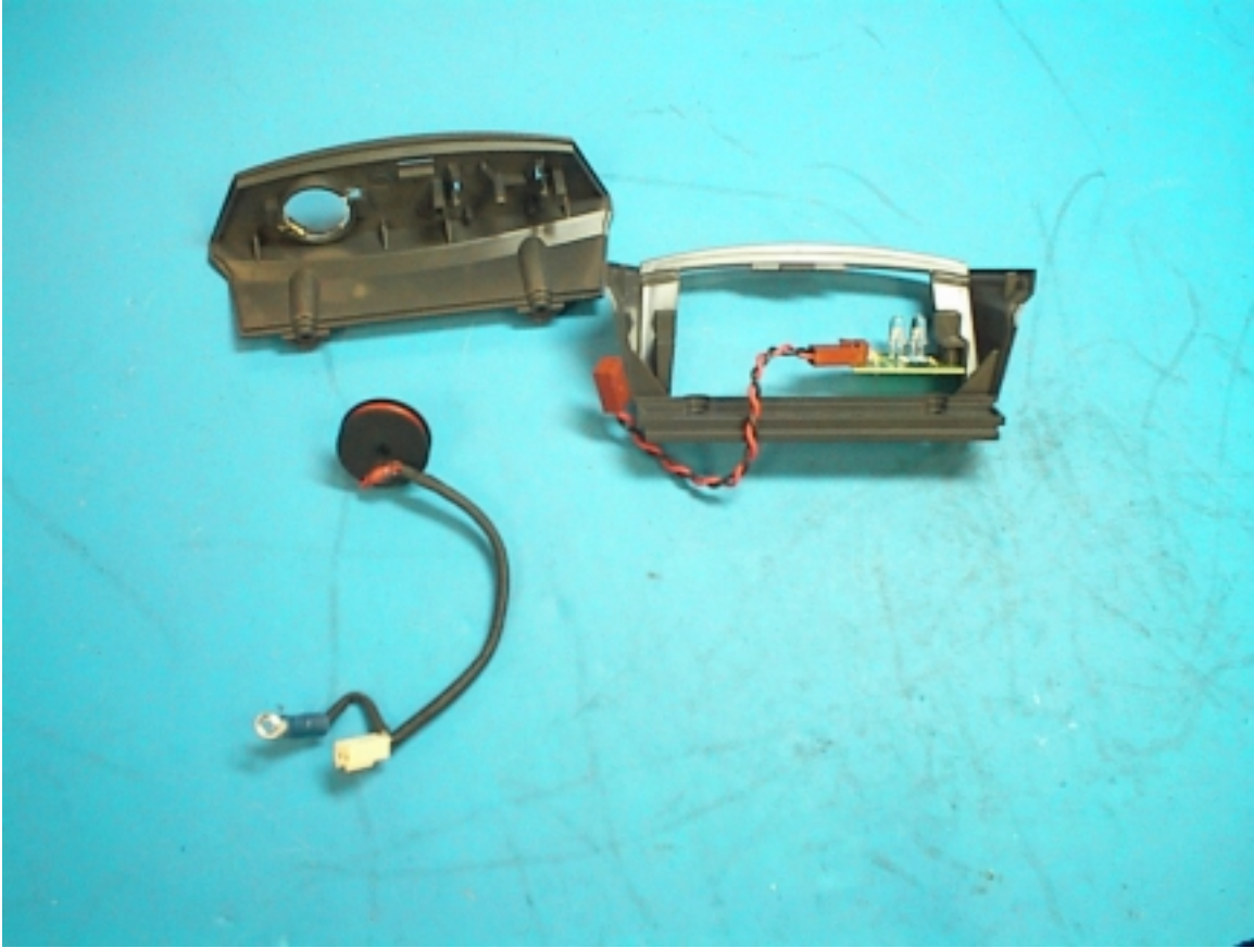
Photo 3 – Antenna and LED board detail
