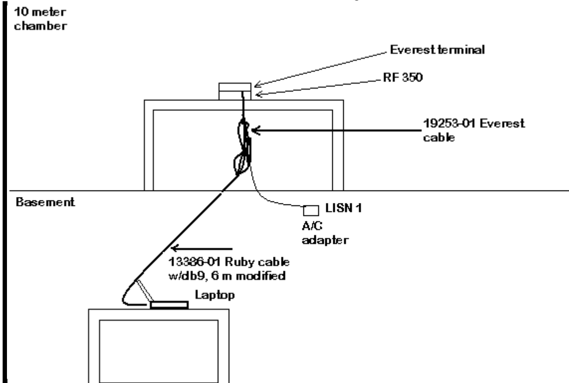
Block diagram
